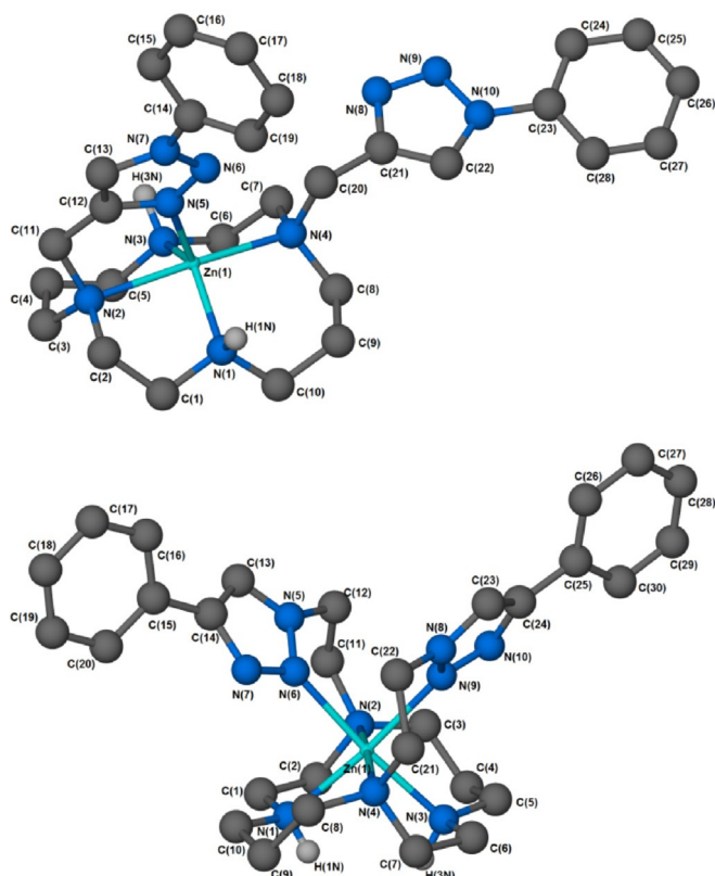
Figure 6. Ball-and-stick depictions of the crystal structures of A ) [\text{Zn}(\mathbf{13})](\text{ClO}_4)_2 and B ) [\text{Zn}(\mathbf{14})](\text{ClO}_4)_2 (exogenous perchlorates omitted for clarity) generated with X-Seed [38] and POV-Ray. [39] Non-hydrogen-bonding hydrogen atoms omitted.
