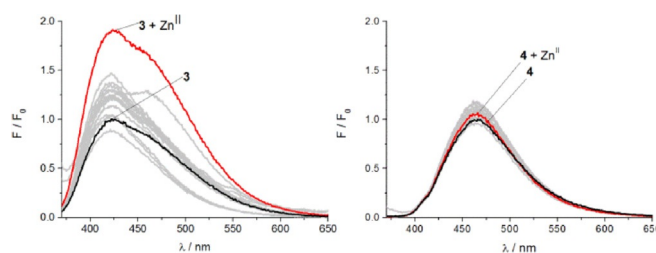
Figure 2. Fluorescence enhancement factors of A) probe 3 (2 μM, λ ex = 350 nm) with different metal ions (20 μM) in HEPES buffer (10 mM, pH 7.4); B) probe 4 (2 μM, λ ex = 357 nm) with different metal ions (20 μM) in HEPES buffer (10 mM, pH 7.4).
