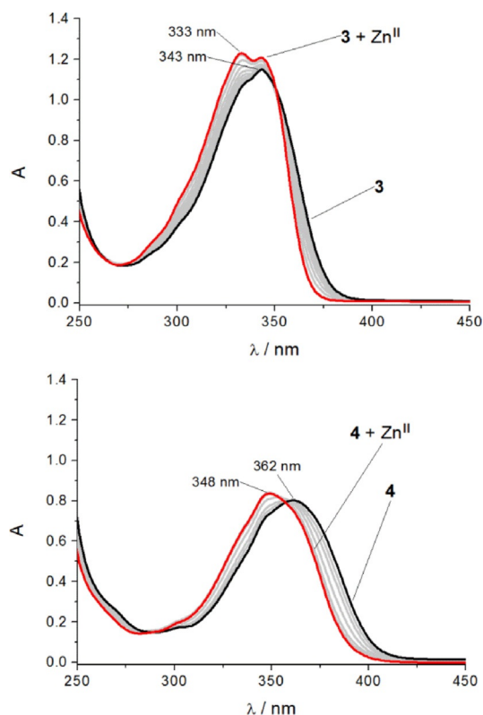
Figure 3. Changes in UV/Vis absorption spectra upon addition of Zn II : A) probe 3 and B) probe 4 (50 μM ligand solution in MeCN, with addition of Zn(ClO 4 ) 2 solution (5 mM in MeCN), added in steps of 0.1 equivalents up to total addition of 1.1 equivalents).
