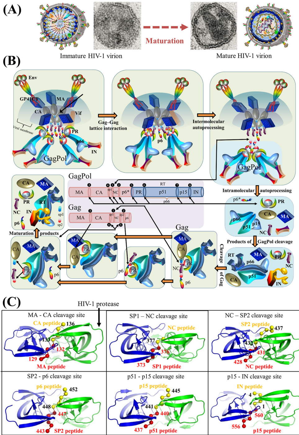
FIG 10 HIV-1 morphology, schematic model of protease-mediated proteolytic processing, and protease-substrate structural complexes. (A) Morphology of HIV-1 immature and mature particles during viral maturation. Schematic models of HIV-1 immature and mature particles are also illustrated. Protease-mediated proteolytic processing triggers the maturation of viral proteins inside HIV particles, resulting in significant changes of virion morphology. Electron micrograph images of HIV virions were obtained from the Centers for Disease Control and Prevention (CDC/Maureen Metcalfe and Tom Hodge; http://phil.cdc.gov/phil/details_linked.asp?pid=13472 ). (B) Protease-mediated proteolytic processing on Gag and GagPol precursors during viral maturation. Five steps have been recorded. First, GagPol dimerization within two GagPol precursors induces the activation of protease dimers with low enzymatic activity (507). Gag and GagPol dimerization occurs before their anchoring to the cell membrane, while GagPol is efficiently packaged into nascent viral particles through its interaction with Gag (621). The transframe region p6* in GagPol prevents premature protease-mediated proteolytic processing (508). The second step is protease-mediated intramolecular ( cis ) autoprocessing. The connection link between SP1 and nucleocapsid is cleaved by protease within the same GagPol dimer (622). The third step is protease-mediated intermolecular ( trans ) autoprocessing. HIV protease in one GagPol dimer further cleaves multiple cleavage sites (NC-p6*, p6*-protease, MA-CA, CA-SP1, protease-p51, protease-p66, p66-integrase, p51-p15, and p15-integrase) in another GagPol dimer (593, 623). After GagPol cleavage, HIV protease, integrase, RT, capsid, and nucleocapsid are folded properly. The fourth step is protease-mediated proteolytic processing of Gag. Mature viral protease cleaves Gag precursors in a specific order: SP1-NC, SP2-p6, MA-CA, CA-SP1, and NC-SP2 (31). This process releases MA, CA, SP1, NC, SP2, and p6 from Gag precursors. In the fifth step, during the maturation of HIV-1 proteins, a series of conformation rearrangements turns immature particles into mature particles (624). Note that protein shapes do not represent the exact protein structures, nor are the protein sizes to scale. (C) HIV-1 protease structures crystallized with 6 substrate peptides derived from Gag and GagPol cleavage sites. Upstream and downstream amino acids of Gag cleavage sites are shown in red and yellow, respectively. See Table S1 in the supplemental material for PDB accession numbers.
