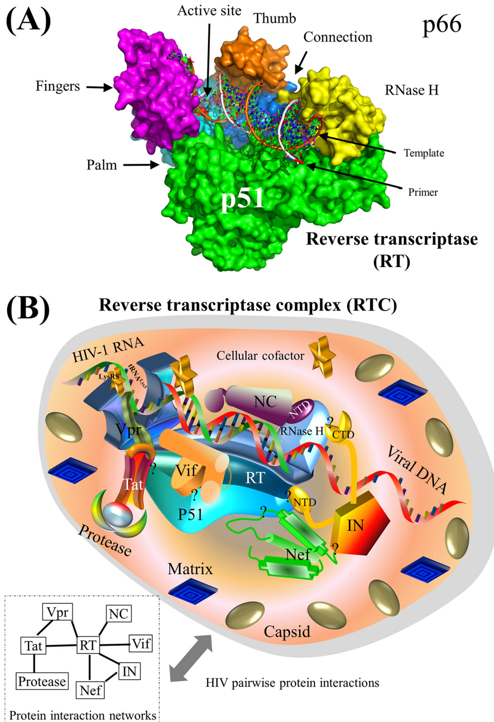
FIG 6 Surface representation of HIV-1 reverse transcriptase and schematic model of the HIV-1 RTC. (A) Surface representation of HIV-1 RT (PDB accession number 3KLG). Two major subunits, p51 and p66, are annotated. The p66 subunit consists of fingers, thumb, palm, connection, and RNase H domains (609). HIV-1 RNA/DNA is shown in the middle, and the active site of RT is mapped to the 3' end of the DNA located between the fingers and thumb domains of HIV-1 RT. See Movie S1 in the supplemental material for a structural movie of HIV-1 RT. (B) Schematic model of HIV-1 pairwise protein interactions in the RTC. The HIV-1 RTC consists of RT, protease, integrase, matrix, capsid, nucleocapsid, Vif, Tat, Nef, Vpr, and many cellular proteins, although the exact composition of the RTC remains debated (93–95). HIV-1 capsid and a subset of phosphorylated matrix are weakly associated with the RTC (95, 96). Seven HIV-1 pairwise protein associations, including the RT-integrase, RT-nucleocapsid, RT-Vif, RT-Tat, RT-Nef, and protease-Tat interactions as well as the RT-tRNA Lys3 -Vpr association, are mapped (Tables 1 and 3). Cellular cofactors (e.g., eEF1A), marked by yellow stars, may interact with the RTC to facilitate HIV-1 reverse transcription (610). Localization of the RTC in the cytoplasm is mediated by the interaction between HIV-1 matrix in the RTC and the actin cytoskeleton (611), although only a small subset of matrix is present in the RTC (95). A protein-protein interaction network is shown at the bottom left to demonstrate the physical protein interactions. Question marks indicate unclear interaction domains. Note that protein shapes do not represent the exact protein structures, nor are the protein sizes to scale.
