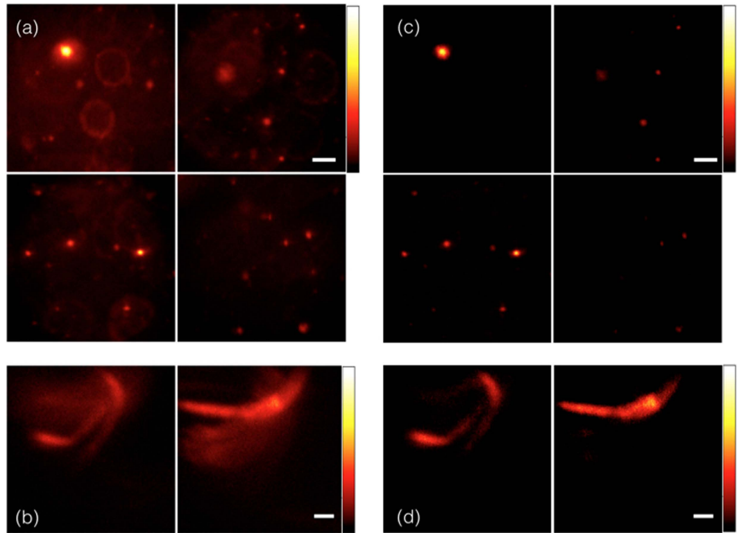
Figure 3. Multi-PSF deconvolution. (a,b) Raw Data. (a) Four focal planes captured by a single camera frame. Each two adjacent planes are separated by 300\mu\text{m} . (b) Two focal planes of one sample which are 200\mu\text{m} apart captured by a single camera shot. Reconstruction results after applying four-PSF deconvolution process in (c) and two-PSF deconvolution process in (d). Sample: (a,c) Randomly distributed 10\mu\text{m} & 500\text{nm} fluorescent beads ( 540/560\text{nm} ) in PDMS. (b,d) C. elegans (GFP labeled). Scale Bar: 40\mu\text{m} . Objective lens: 10\times/0.25 .
