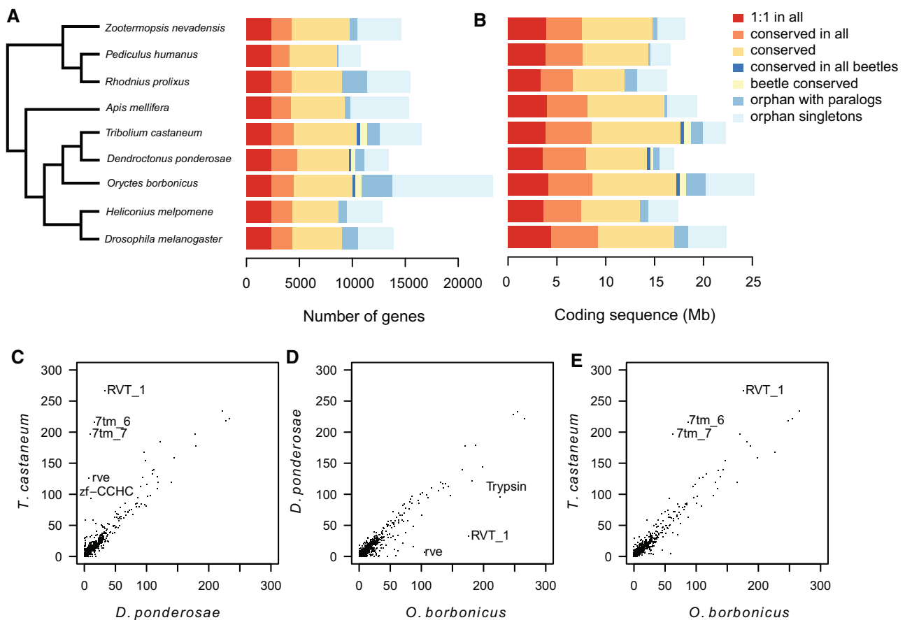
Fig. 1. —Conserved and lineage-specific patterns of gene content evolution. (A) Schematic phylogeny of investigated insect genomes (Hunt et al. 2007; Trautwein 2012) and distribution of genes in different orthology classes. (B) Amount of coding sequence in different orthology classes. (C–E) Protein domain (PFAM) count comparison between all three beetle genomes. Large protein domain families that show the most extreme differences in gene counts are labeled in each comparison.
