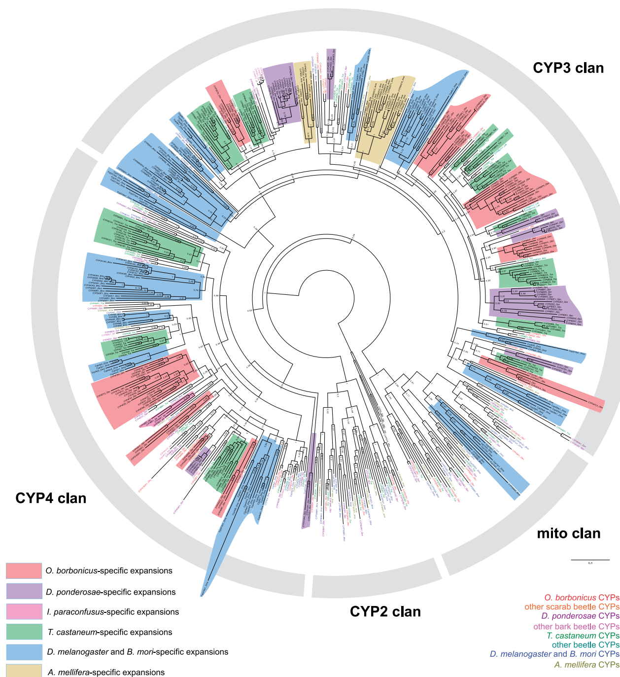
Fig. 3. —A maximum-likelihood tree of insect CYPs. The tree was calculated under the LG+G model, and is rooted by CYP51 sequences. A linear version of the tree is available in supplementary figure S9, Supplementary Material online.
