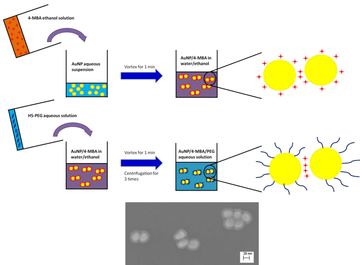
Schematic 1. Production of AuNP/4-MBA/PEG nanosensor
