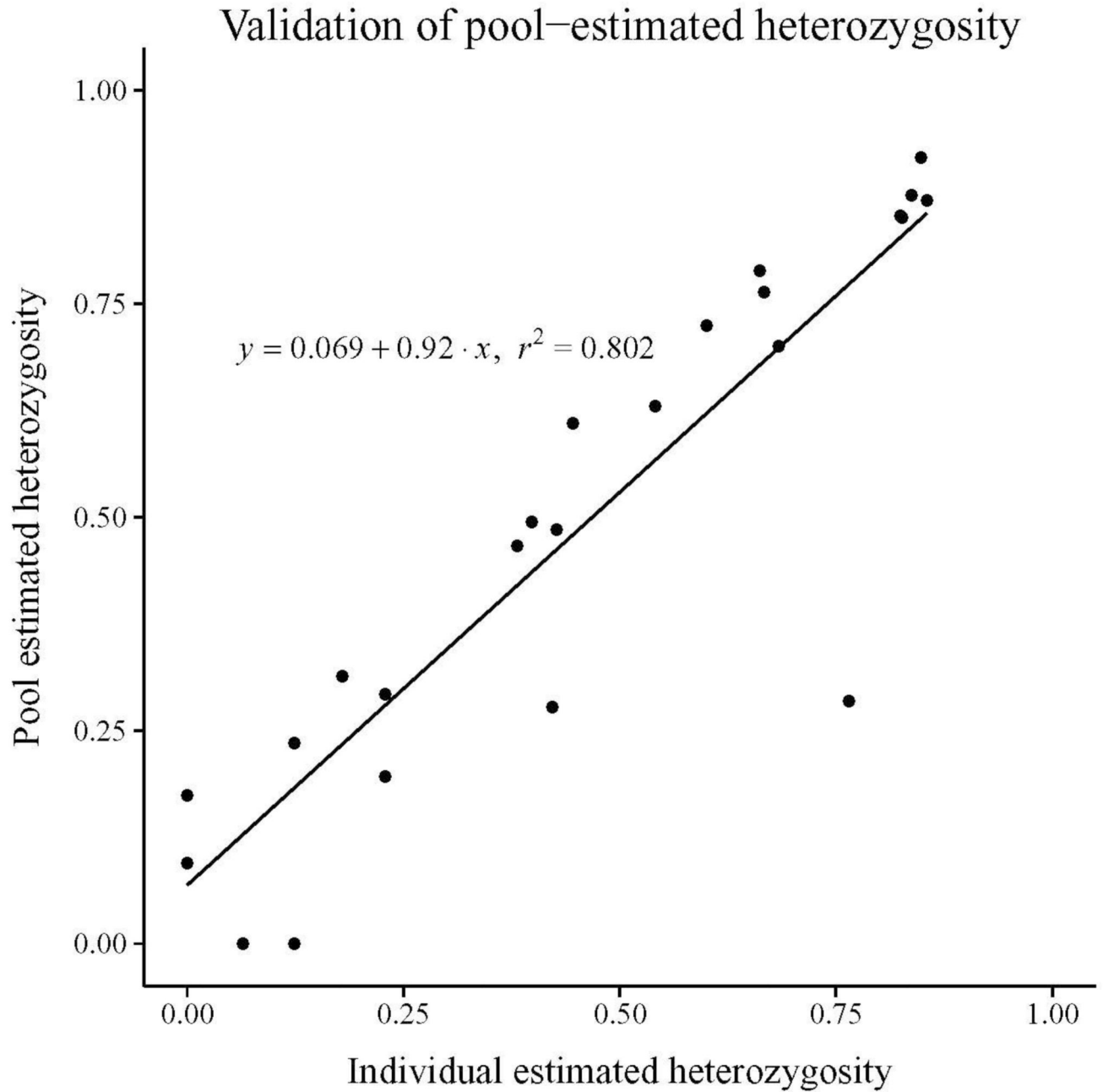
Figure 1. Validation of heterozygosity estimation from pooled samples
