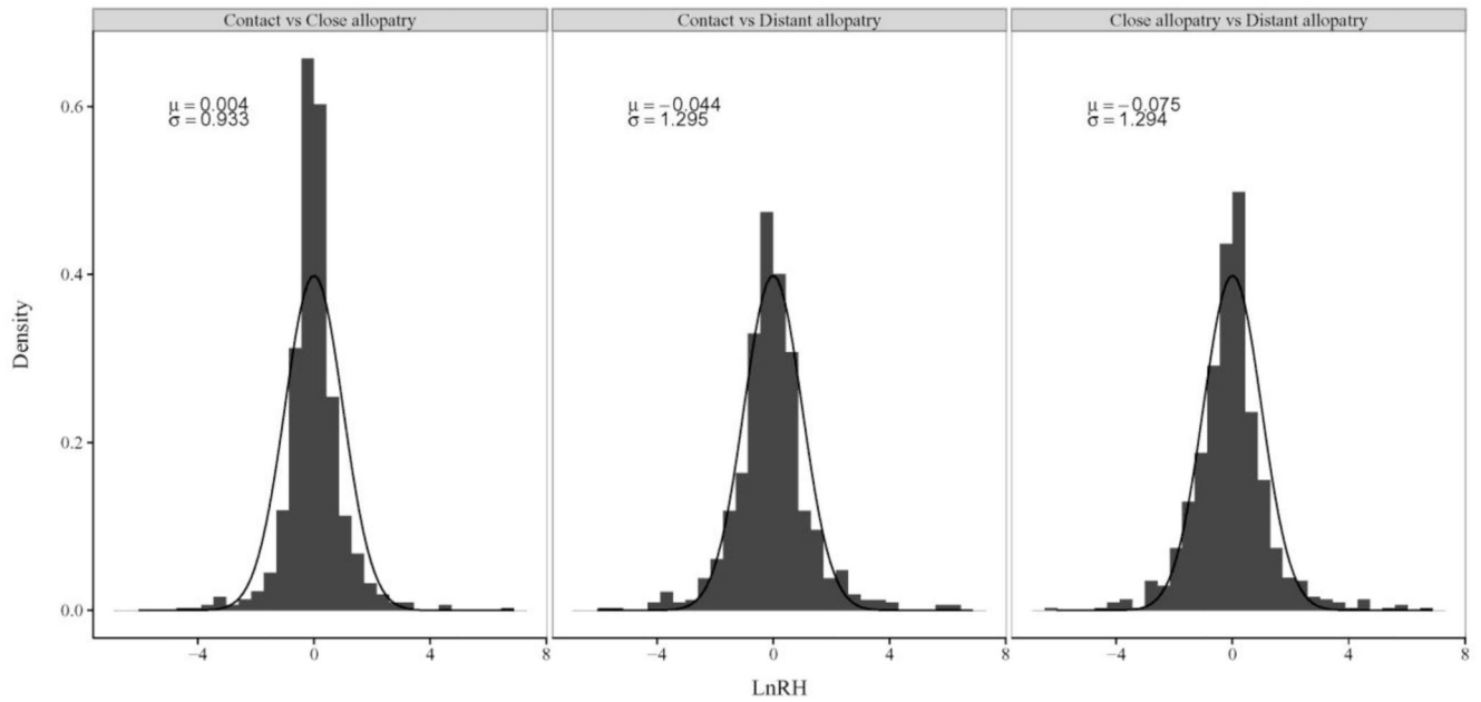
Figure 2. \ln RH distributions for the three pairwise sample comparisons
