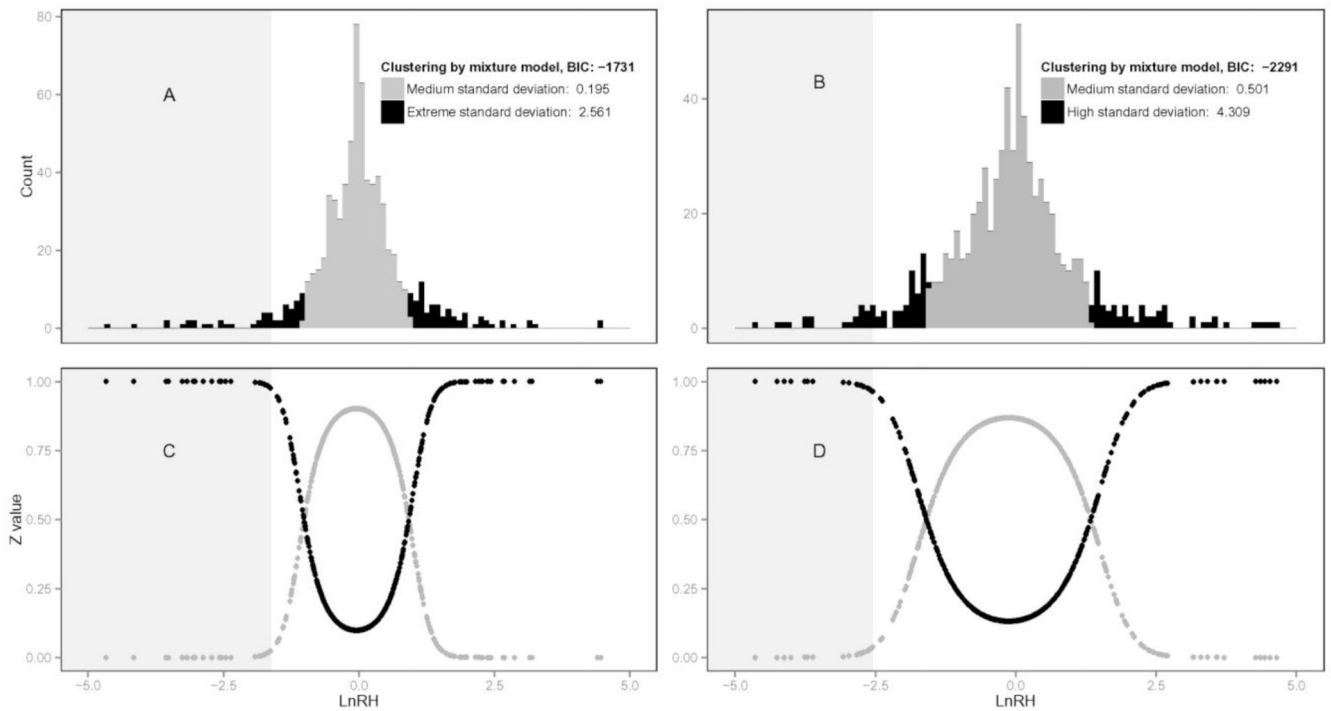
Figure 3. Clustering by mixture models of \ln RH distributions
