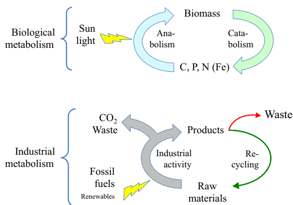
Fig. 2. Biological metabolism versus industrial metabolism. The upper part of the figure sketches the basic metabolic cycle of the biosphere: a sustainable sequence of biochemical reactions for building (anabolism) and dismantling (catabolism) biomass and other bio-compounds on the basis of available C, N and P species (and to a lesser extent others like Fe etc.) obtainable in the biosphere. The lower part outlines in a super-simplified form the action of the so-called Industrial metabolism (Ayres, 1994). This involves the integrated collection of human-made physical and chemical processes that transform raw materials and (generally non-renewable) energy into products, leaving wastes, e.g. CO 2 and recalcitrant products and materials) along the way. The interplay between biological cycles and industrial processes at global scale was a popular topic in the late 1970s (de Rosnay, 1979). Alas, the current state of affairs makes such an industrial metabolism – and it is associated industrial ecology (Allenby, 2006) ultimately unsustainable. The notion of transmetabolism discussed in this article attempts to overcome the breach between the natural and the human-made chemical domains by bridging the two with new reactions and rationally delivering them at a global scale by means of deeply engineered biological agents.
