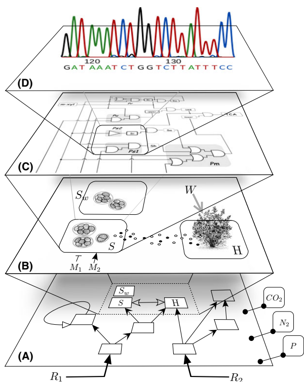
Fig. 1. At least four scales need to be addressed for knocking-in a new functionality within a pre-existing ecological web: (A) the ecosystem level, characterized by interactions among species (S, H), external inputs/resources (R) in a biogeochemical context e.g. \text{CO}_2 , \text{N}_2 and P availability. (B) the pair-wise species interplay level, which may encompass transactions between actors of different kingdoms (microbial, plants, animals), specially mutualistic interactions, the components of which can be affected positively and negatively by external signals (M), water (W) being paramount in the whole setup. (C) the genetic, epigenetic and biochemical circuit level that rules the behaviour of single-species following a logic network (the logicome ) and (D) the specific DNA sequence necessary to make the biological or chemical activity of interest happen (Solé, 2015).
