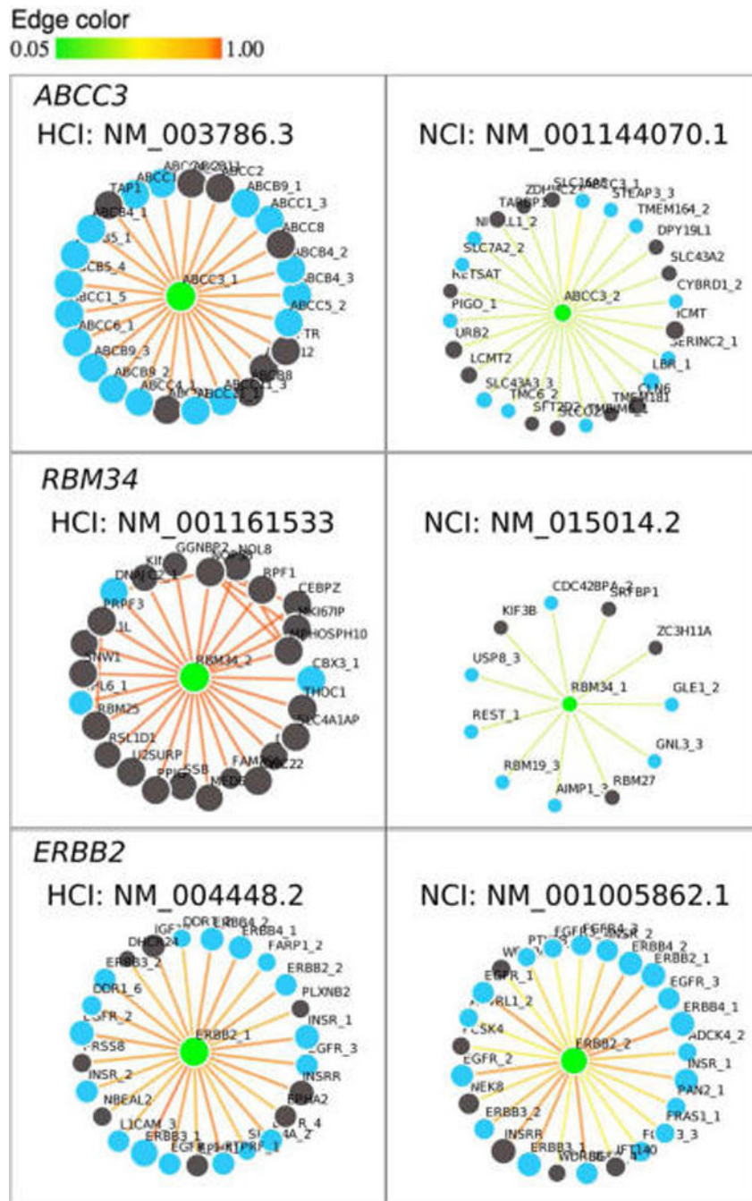
Figure 2. Illustrations of the HCI and NCI using the ABCC3 (ATP-Binding Cassette, Sub-Family C (CFTR/MRP), Member 3, chr17:48,712,205–48,769,063), RBM34 (RNA binding motif 34, chr1:235,131,183–235,161,616), and ERBB2 (erb-b2 receptor tyrosine kinase 2, chr17:37,844,167–37,884,915) genes. For each gene, the isoform with higher AFR score is selected as HCI. Black and blue nodes represent single-isoform and multi-isoform genes, respectively; green nodes indicate the queried gene/isoform. Gene names followed by numbers indicate isoforms for easily recognizing the originating-gene, which are
