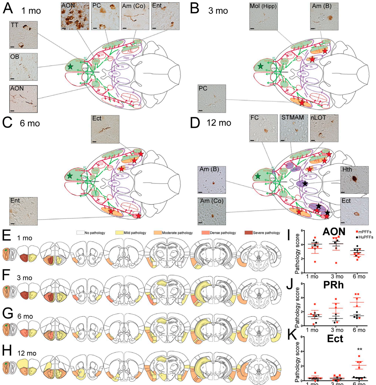
Figure 4. HuPFFs inoculated in OB led to slower progressive spreading of \alpha -syn pathology first to olfactory structures, and then to connected brain. (A–D) Schematic of a ventral brain view, depicting the localization of pathology (Pser129) at 1, 3, 6, and 12 mo after huPFFs injections. Micrographs show pathology (Pser129) in related brain regions. (A–E) Histochemical analysis was performed on all animals from the 1-, 3-, 6-, and 12-mo survival time points. The sections were immunostained in eight independent histochemical experiments. 1 and 3 mo delay, n = 4 mice per group; 6 and 12 mo delay, n = 5 mice per group. (A) At 1 mo delay, pathology was observed in olfactory regions (Ipsi AON, Pc, Am Co, Ent, TT, OB, and contra AON). Bar, 10 \mu m. (B) At 3 mo delay, pathology appeared in a few more ipsilateral (Mol and Am B) and contralateral brain regions (PC). Regions located one synapse away from the olfactory system are identified with a red star. (C) Pathology appeared in two additional brain regions after 6 mo. (D) 12 mo after injection, additional brain regions show pathology; Regions located 2 synapses away from the olfactory system are identified with black stars. (E–H) Diagram illustrating the anatomical pattern of \alpha -syn pathology in the brain on coronal sections, 1 mo (E), 3 mo (F), 6 mo (G), and 12 mo (H) after injection. (I–K) Scoring of Pser129 immunoreactivity (neurites and cell bodies) in the AON (I), the perirhinal (PRh; J), and ectorhinal cortex (Ect; K). Scoring was performed on all animals from the 1-, 3-, 6-months survival time points. Sections were immunostained in eight independent histochemical experiments (1 and 3 mo delay, n = 4 mice per group; 6 mo delay, n = 5 mice per group) and were analyzed by two-way ANOVA, followed by a Tukey post-hoc test. Statistics are provided in Table S4. **, P < 0.05 .
