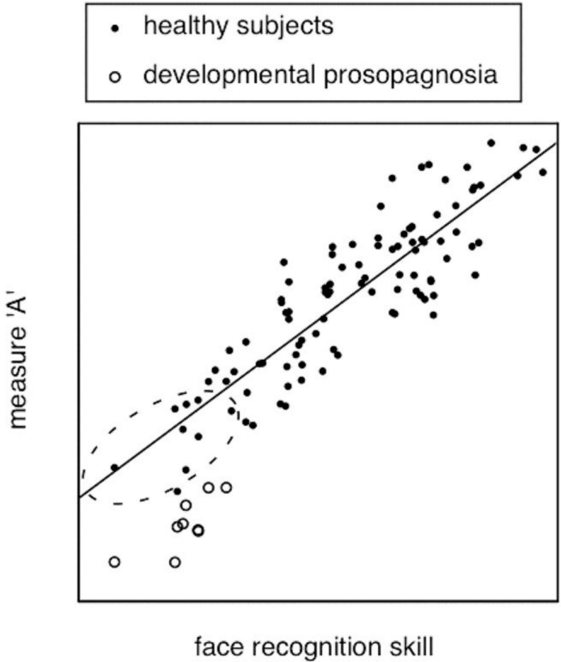
Figure 2. A hypothetical qualitative difference in perceptual performance that might distinguish developmental prosopagnosia from those bad at faces. Suppose that there is some perceptual measure A that is a linear function of face recognition skill in the normal population, so that those on the low end of the normal distribution still follow this linear function. If the developmental prosopagnosic subjects performed worse on measure A than predicted by the
