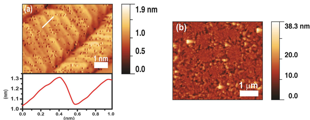
Figure 7. Topographic AFM images of the annealed films at 800 °C: (a) Pure TiO 2 , with height profile of the atomic terraces and (b) 0.16Ag-TiO 2 .
