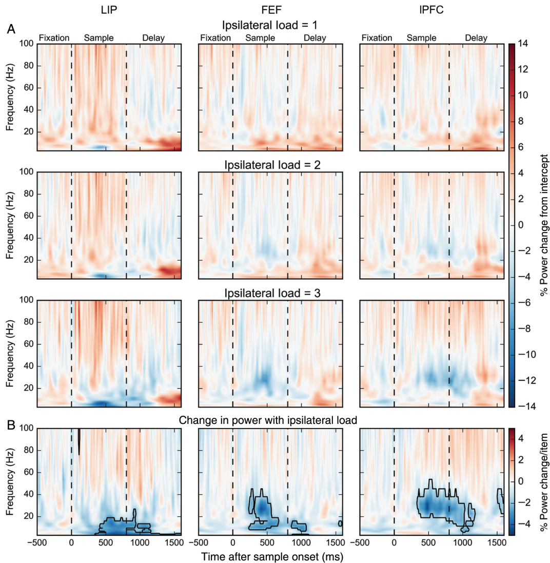
Figure 3. (A) Percent power change for ipsilateral loads 1, 2, and 3 relative to the model intercept across frequencies and time. (B) Percent power change per ipsilateral stimulus. Boxes indicate significant modulations (bootstrap Z-test, P < 0.05 , Holm corrected for 22 frequencies \times 211 time points).
