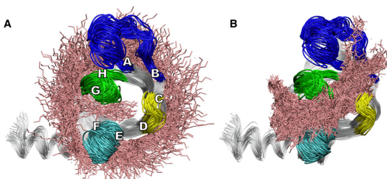
Figure 5. Plausible Routes of Ligand Entry and Exit to and from the PagP Binding Site Based on Steered MD Simulations
