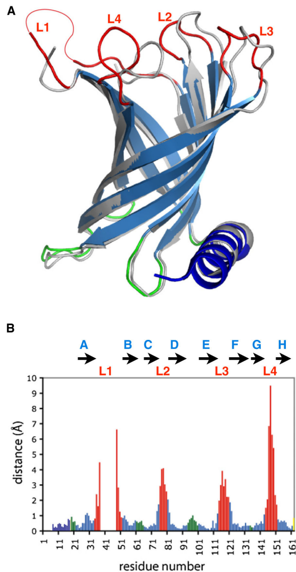
Figure 2. Differences between the SDS/MPD and the LDAO Crystal Structures of PagP (A) Superposition of the SDS/MPD (blue, red, green) and LDAO (gray) crystal structures of PagP. The thin red line in L1 connects residue 37 to 46 and indicates the disordered region of this loop. Only the \beta sheet residues were used in the least-squares fitting. (B) Distances between the \alpha carbons of the SDS/MPD and the LDAO crystal structures of PagP. Residues in \beta strands are in blue, and only those were used for the superposition. The N-terminal helix is shown in dark blue, the periplasm-facing loops are in green, and the extracellular loops L1–L4 are in red. See also Figure S1.
