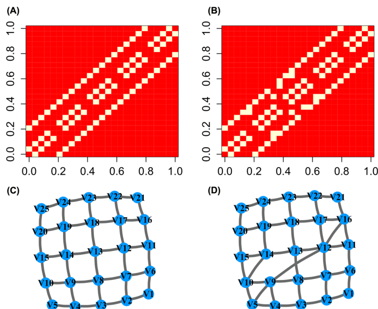
Fig. 5 Results of fitting an Ising model to simulated multivariate binary data. The true simulated grid is plotted in (a) and (c). The estimated graph structure via XMRF ( . . . , method="ISM" ) is plotted in (b) and (d)
