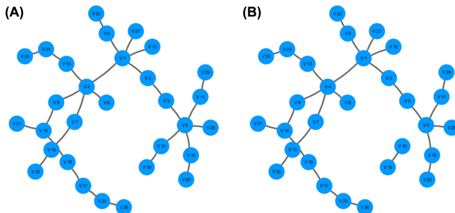
Fig. 7 Simulated network from XMRF ( Sim(..., model="LPGM") ) (a) and inferred network estimated via XMRF ( ... , method="LPGM" ) with network sparsity determined via stability selection (b)
