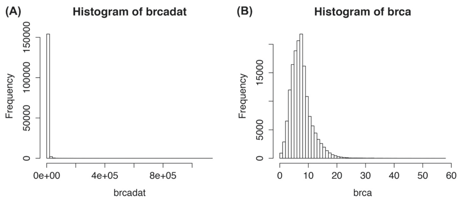
Fig. 1 Distribution of TCGA BRCA RNA-Seq data before (a) and after (b) preprocessing. The latter gives a distribution more appropriate for Poisson family graphical models
