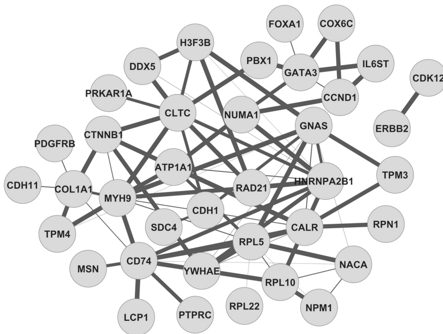
Fig. 2 Inferred relationships between cancer census genes from TCGA breast cancer patients. The width of edges reflects the strength of inferred relationships
