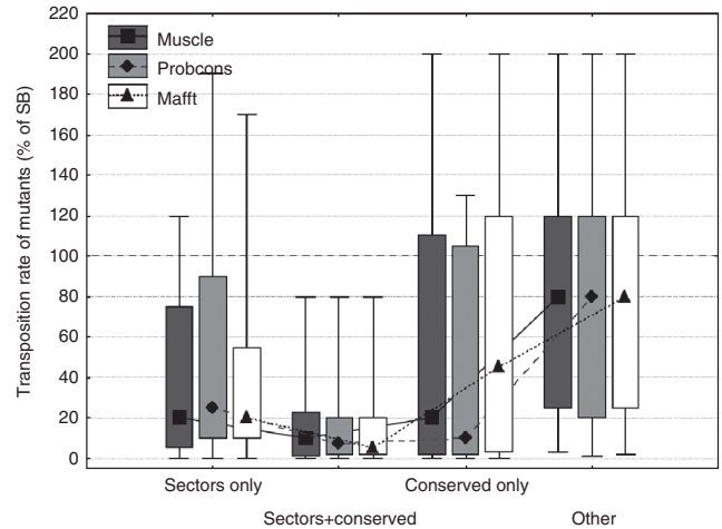
Figure 3 The effect of sectors on transposition rate is not a by-product of positional conservation. Sector and conserved residues were split into three groups: sector residues with low positional conservation ( D < 0.5 ), sector residues with high positional conservation, and conserved residues that are not part of any sector. Transposition rates of mutants (median, box: 25–75%, whiskers: 10–90%) in all three groups are significantly different from mutants in other residues ( P < 0.05 for all comparisons, Fisher post-hoc tests, analysis of variance on log transformed transposition rates), and there is no significant difference between the mutants of nonconserved sector and conserved but non-sector residues ( P > 0.05 in all three alignments, Fisher post-hoc tests).
