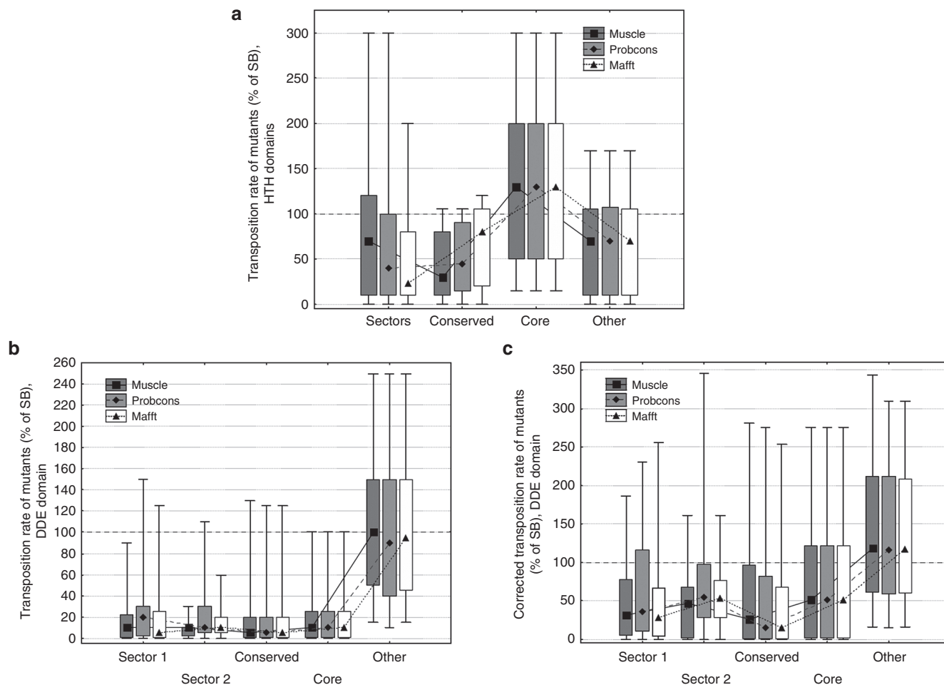
Figure 5 The effect of residue location on transposition rate, in the two regions of the protein (median, box: 25–75%, whiskers: 10–90%). (a) In the HTH-region, mutants of sectors, conserved or buried residues are not significantly different from the remaining mutants ( P > 0.05 for all comparisons, Mann-Whitney U -tests). (b) In the DDE domain the differences are highly significant ( P < 0.05 for all comparisons, Mann-Whitney U -tests), even after correcting for the different effects of free energy of folding (c) . Note that in the DDE domain 50% of mutants of “other” residues are characterized with higher activity than the wild type SB.
