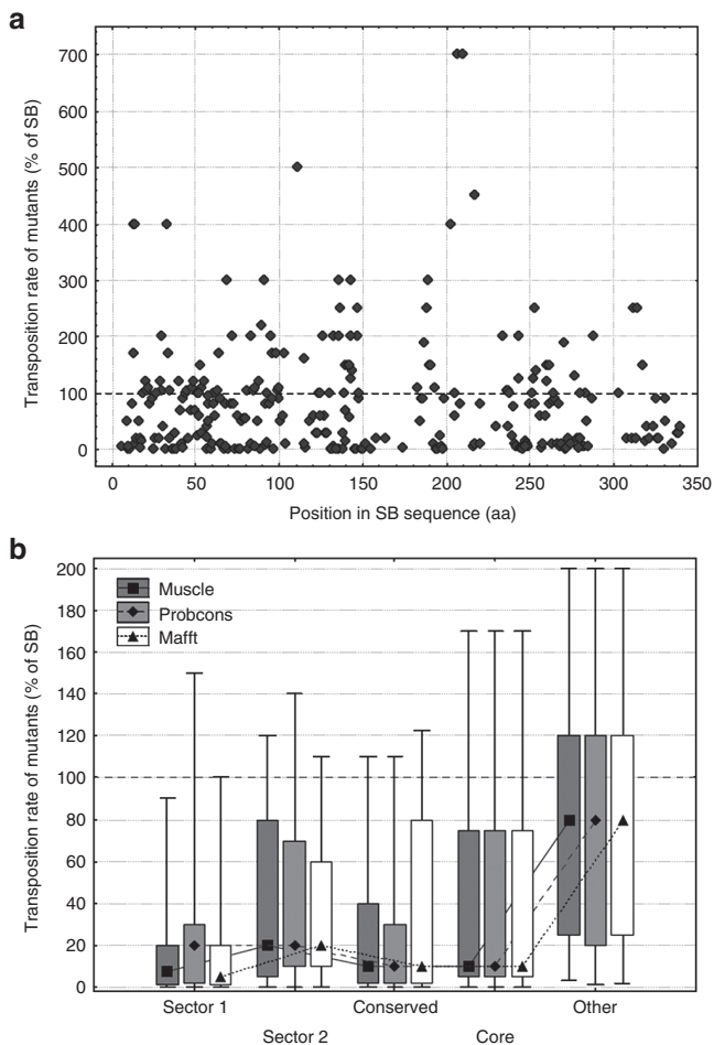
Figure 2 Effect of residue location on the transposition rate of SB mutants. (a) The location of the mutations along the SB transposase sequence, and their effect on transposition rate. The 286 mutants are distributed approximately evenly across the sequence; the majority of mutants reduces transposition rate ( < 100\% of SB). None of the Pfam conserved domains show a clear difference from the rest of the sequence. (b) The effect of sectors, conserved residues and protein core on transposition rate (median, box: 25–75%, whiskers: 10–90%). Mutants in both sectors, conserved residues and residues of the protein core have significantly lower transposition rates than other residues, irrespectively of the aligner used ( P < 0.05 , Mann-Whitney U -tests).
