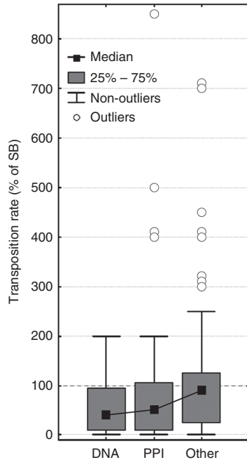
Figure 6 The effect of DNA-protein and protein-protein interactions on transposition rate. When outliers are excluded, mutants of residues interacting with DNA (“DNA”) and the other SB chain (“PPI”) have significantly lower transposition rates ( P < 0.05 , Mann-Whitney U -test) than other residues located at the surface ( RSA > 0.1 ). Surprisingly, 12 of the 14 hyperactive mutants (outliers, 300+% activity) are also located in the protein surface, and none in the DNA binding regions, suggesting that the modification of protein-protein interactions might be responsible for their dramatically increased activity. (Outliers with identical transposition rates were shifted by 10%, for visibility)
