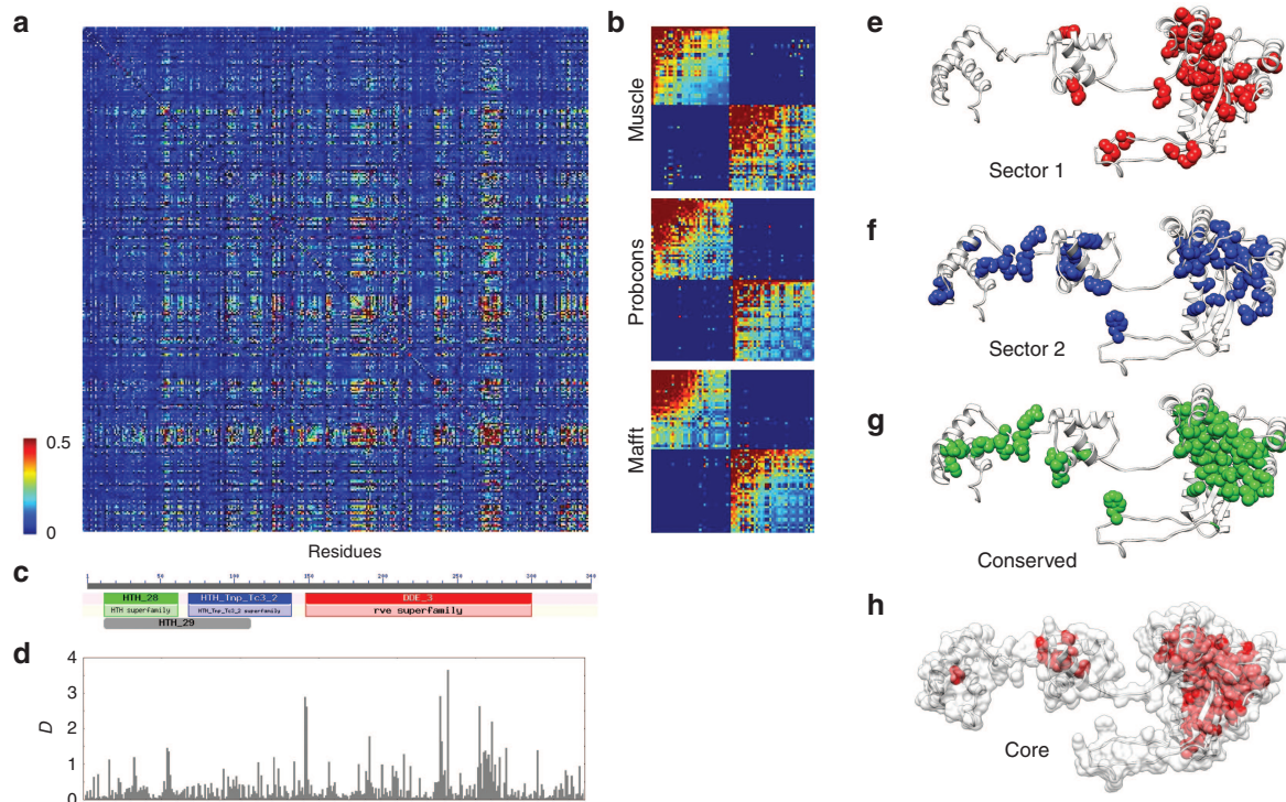
Figure 1 Identification of sectors and conserved domains in the Sleeping Beauty (SB) transposase. (a) Statistical Coupling Analysis (SCA) matrix for the muscle alignment of 289 homologous sequences present in RepBase (+SB). The matrix represents correlations between amino acid frequencies at each position of the alignment, i.e. , residue pairs that coevolve. (b) Cleaned SCA matrices for three alignments made with muscle , probcons , and mafft aligners, containing the residues of the two sectors. Residues within sectors show correlated evolution, while there is almost no correlation between sectors. (c) The transposase contains three Pfam conserved domains; two HTH domains with DNA binding functions, and a DDE domain with endonuclease activity. (d) The distribution of conservation scores ( D ) across the sequence. (e,f) The location of the two sectors identified with the muscle alignment in the tertiary structure of the SB transposase. The sectors are located across secondary structure elements, and are less compact than the ones reported so far, possibly due to the low sequence similarity in the alignments. Both sectors have residues in multiple conserved domains; most notably sector 2, which has residues in all three Pfam domains of the protein. (g) The location of the conserved residues ( D > 0.5 , muscle alignment, see also Supplementary Table S2 ) of the transposase. (h) The residues of the protein core. All residues with relative solvent accessibility below 0.1 are highlighted with red.
