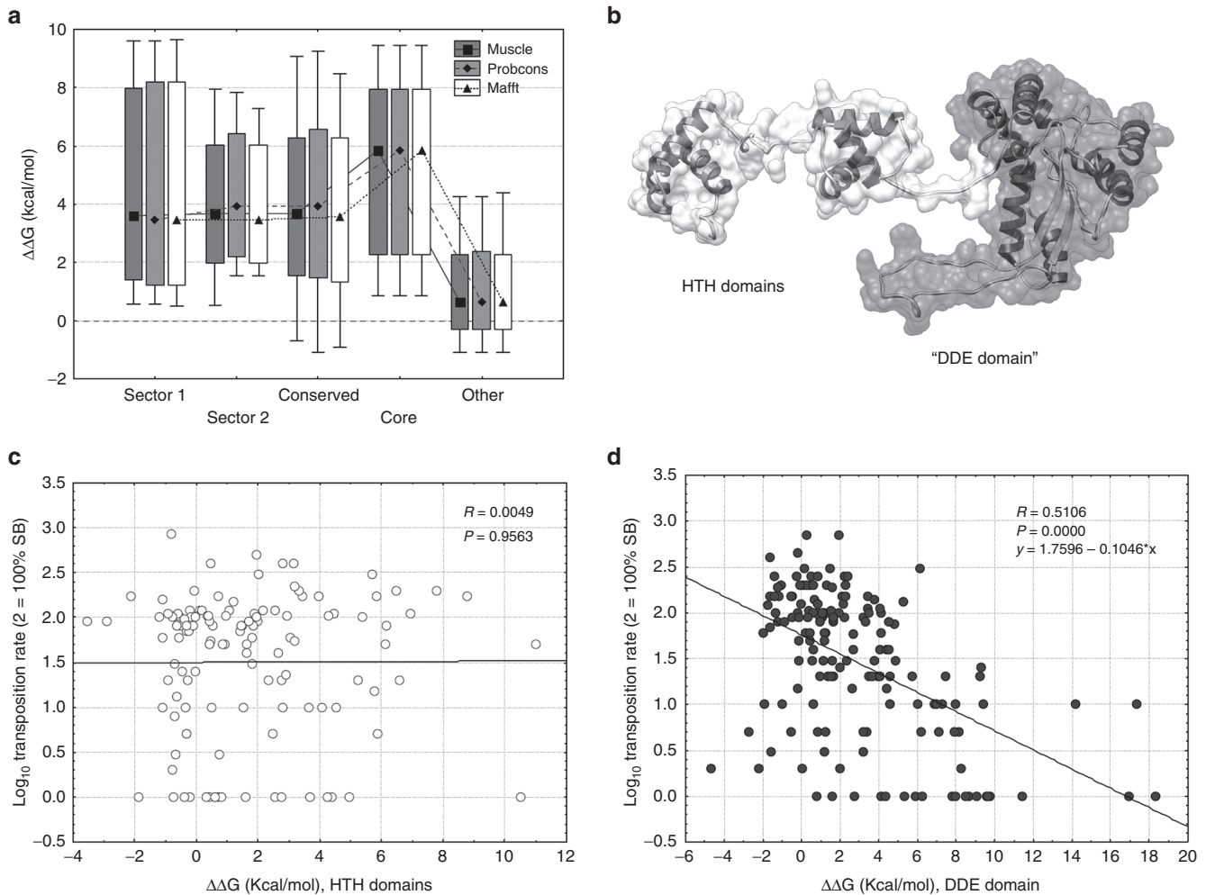
Figure 4 The effect of mutations on the change of the free energy of unfolding (median, box: 25–75%, whiskers: 10–90%). (a) Mutations in sectors and the core are significantly more destabilizing ( \Delta\Delta G > 0 ) than mutants of other residues ( P < 0.05 for all comparisons, t -tests). (b) The monomer of SB. The flexible N-terminal arm of the protein containing the HTH domains (residues 1–120) is indicated with white, the globular part (residues 121–340), which contains the DDE domain, with gray. (c) In the flexible arm the effect of mutations on \Delta\Delta G is not correlated with transposition rate ( P = 0.95 ). (d) In the globular region we find a significant negative correlation ( P < 0.001 , R = -0.51 ) between \Delta\Delta G and transposition rate.
