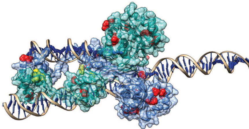
Figure 7 The location of the 14 hyperactive mutations in the SB dimer. Yellow residues represent mutants in protein-protein interfaces, red residues other mutants. As SB probably forms also a tetramer in certain phases of transposition, the number of residues taking part in protein-protein interactions is probably higher. (See also the supplementary “hyperactive.py” Chimera file.)
