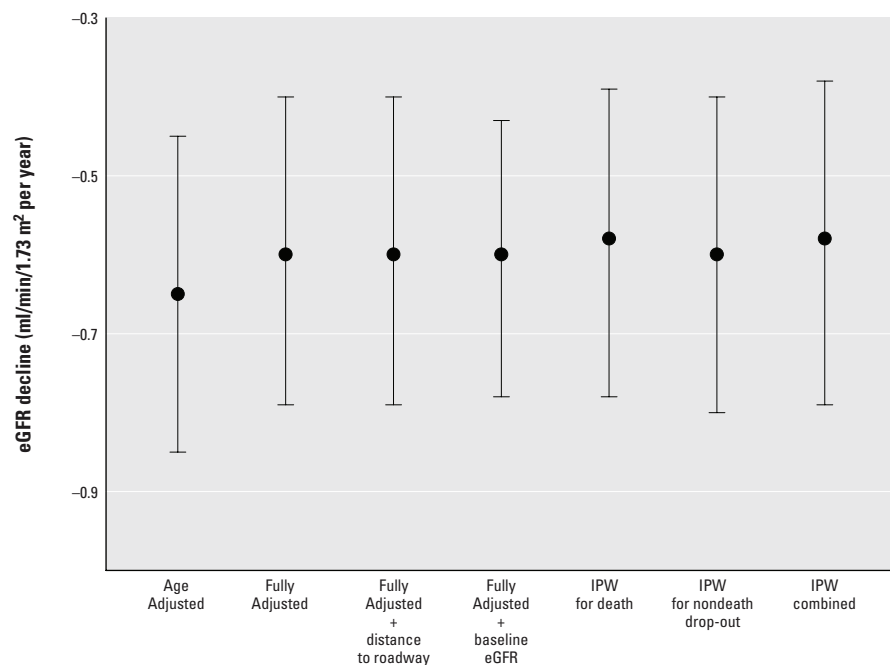
Figure 4. Adjusted difference in annual change in eGFR since first visit (mL/min/1.73 m 2 /year) per 2.1 \mu\text{g}/\text{m}^3 interquartile range increase in 1-year PM 2.5 . Associations were estimated in time-varying linear mixed-effect models of eGFR with random intercept for study participant. Age-adjusted models included adjustment for time since first visit and age at first visit. Fully adjusted models included additional adjustment for BMI, total cholesterol, diabetes, coronary heart disease, ARB medication, ACEI medication, other anti-hypertensive medication, years of education, percentage below poverty level in census tract, parental homeownership, smoking status, cumulative pack-years smoked, and daily alcohol intake. For the fully adjusted model, we also adjusted for distance to roadway and baseline eGFR and applied stabilized IPW for censoring by death and nondeath dropout and for the combination of both censoring mechanisms. The effect estimates presented for each model were estimated from the interaction between time since first visit and 1-year PM 2.5 .
