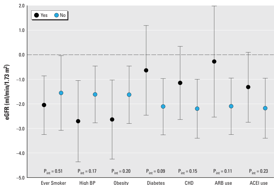
Figure 3. Adjusted differences in eGFR per 2.1 μg/m 3 interquartile range increase in 1-year PM 2.5 in subgroups according to participant characteristics. Associations were estimated in time-varying linear mixed-effect models of eGFR with random intercept for study participant after adjustment for time since first visit, age at first visit, BMI, total cholesterol, diabetes, coronary heart disease, ARB medication, ACEI medication, other anti-hypertensive medication, years of education, percentage below poverty level in census tract, parental homeownership, smoking status, cumulative pack-years smoked, and daily alcohol intake. Effect estimates presented for each subgroup were estimated from the nested interaction model. Abbreviations: ACEI, angiotensin converting enzyme inhibitor; ARB, angiotensin receptor blocker; BP, blood pressure; CHD, coronary heart disease; eGFR, estimated glomerular filtration rate; P int = p -value for interaction; PM 2.5 , fine particulate matter ≤ 2.5 μm in diameter.
