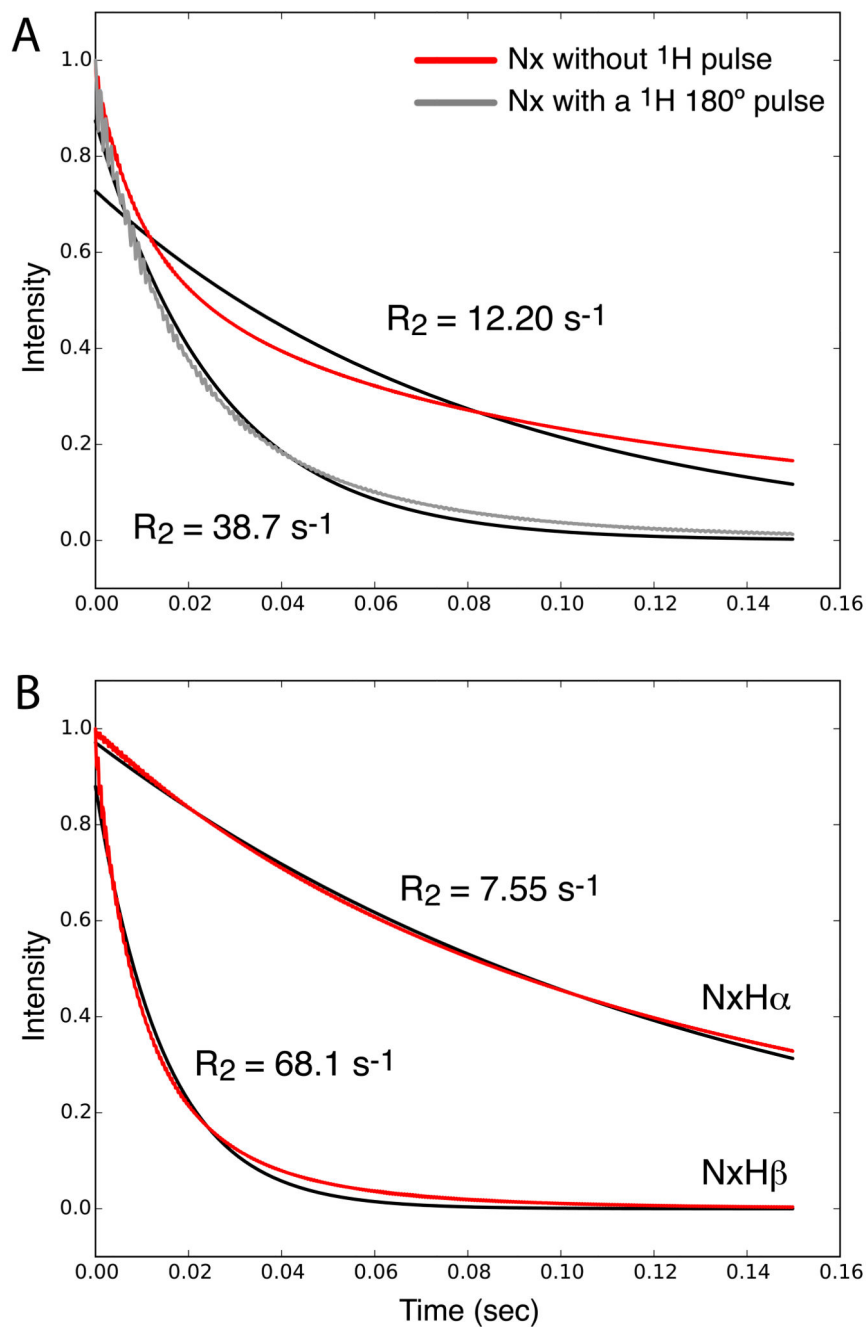
Figure 1. Simulated evolution of ^{15}\text{N} spin coherences under a spin-lock RF field. (A) Time evolution of in-phase N_x coherence (red) and a single-exponential fit, which clearly results in poor agreement with the decay. For the simulation shown in grey, a ^1\text{H} \pi pulse was inserted in the center of the spin-lock period. An exponential fit is shown in black. (B) Simulation of the doublet components, N_x\text{-}[\text{H}^\alpha] , N_x\text{-}[\text{H}^\beta] (red), and exponential fits (black). The jump angle was 20 degrees and the jump rate constant 30000\text{ s}^{-1} .
