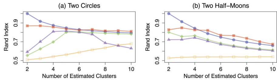
Fig 5. Simulation results for the two circles and two half-moons clusters with n = 100 , averaged over 200 data sets. Line types are as described in Figure 2.
