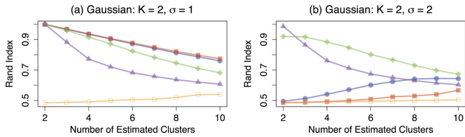
Fig 2. Simulation results for Gaussian clusters with K = 2 , n = p = 30 , averaged over 200 data sets, for two noise levels \sigma = \{1, 2\} . Colored lines correspond to single linkage hierarchical - clustering (—●—●—●—), average linkage hierarchical clustering (—◆—◆—◆—), k-means clustering (1074i03), convex clustering with q = 1 (—□—□—□—), and convex clustering with q = 2 (—▲—▲—▲—).
