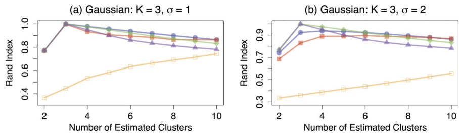
Fig 3. Simulation results for Gaussian clusters with K=3 , n=p=30 , averaged over 200 data sets, for two noise levels \sigma = \{1, 2\} . Line types are as described in Figure 2.
