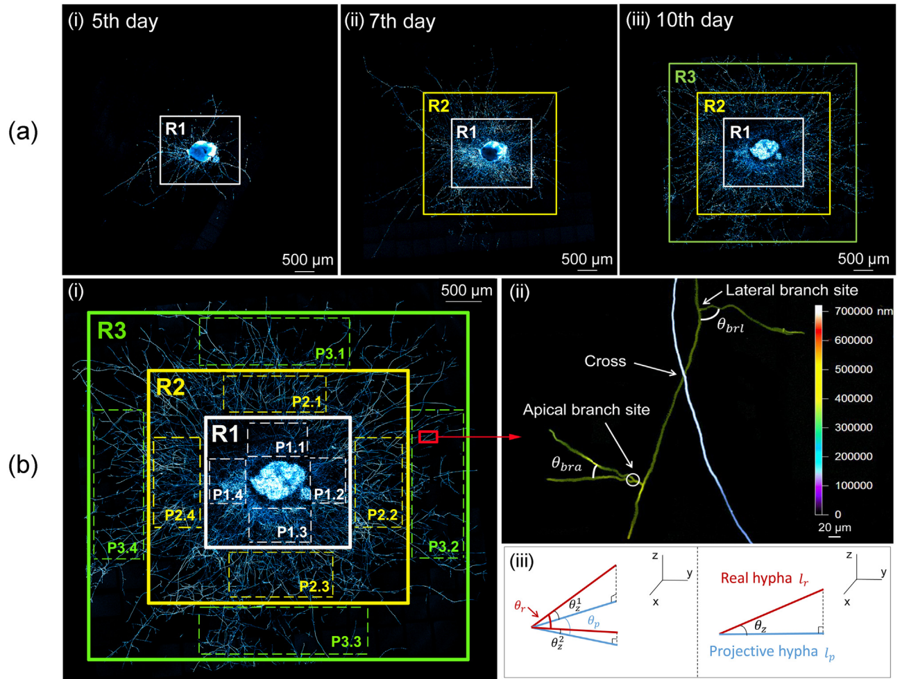
Fig 1. Method of the measurement of branching characteristics. (a) Three regions with equal gap to partition the young and old hyphae: (i) R1, (ii) R2 and (iii) R3, covering almost the entire colony on the 5th, 7th and 10th day following inoculation. (b) (i) Four portions selected for the measurement in each of the three regions (e.g., P1.1, P1.2, P1.3 and P1.4 in R1). (ii) Zoom of a color projection for measurement to show a cross of two hyphae with two types of branch sites and branch angles (AB angle ( \theta_{bra} ) and LB angle ( \theta_{brl} )). The color bar shows the depth of the mycelium along the z-axis. (iii) Errors between real values and projective ones caused by z-direction growth of hyphae: (left) real branch angle ( \theta_r ), projective branch angle ( \theta_p ), and angle of the real hypha to the xy plan ( \theta_z ); (right) real branch length ( l_r ) and projective branch length ( l_p ).
