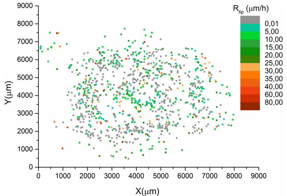
Fig 4. Spatial distribution of tip extension rate ( R_{tip}(i; x, y) ) during 17 days of observations. (x, y) are the coordinates of the position of tip i . The colors display the different ranges of rate: from green, less than 25 \mu\text{m}/\text{h} , to orange for the > 25 \mu\text{m}/\text{h} . Grey points represent dormant tips.
