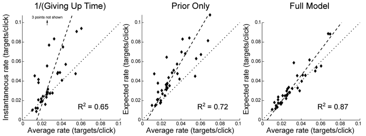
Figure 9. Plots of participants’ median rate when quitting trials vs. their average rates in Experiment 2, for various models. The dotted line indicates the identity (1:1) line: if participants left the patch when their expected rate was exactly the average rate, then all dots would lie along this line. Dashed lines are the best linear fit to the data; R 2 for each fit is given on the graph.
