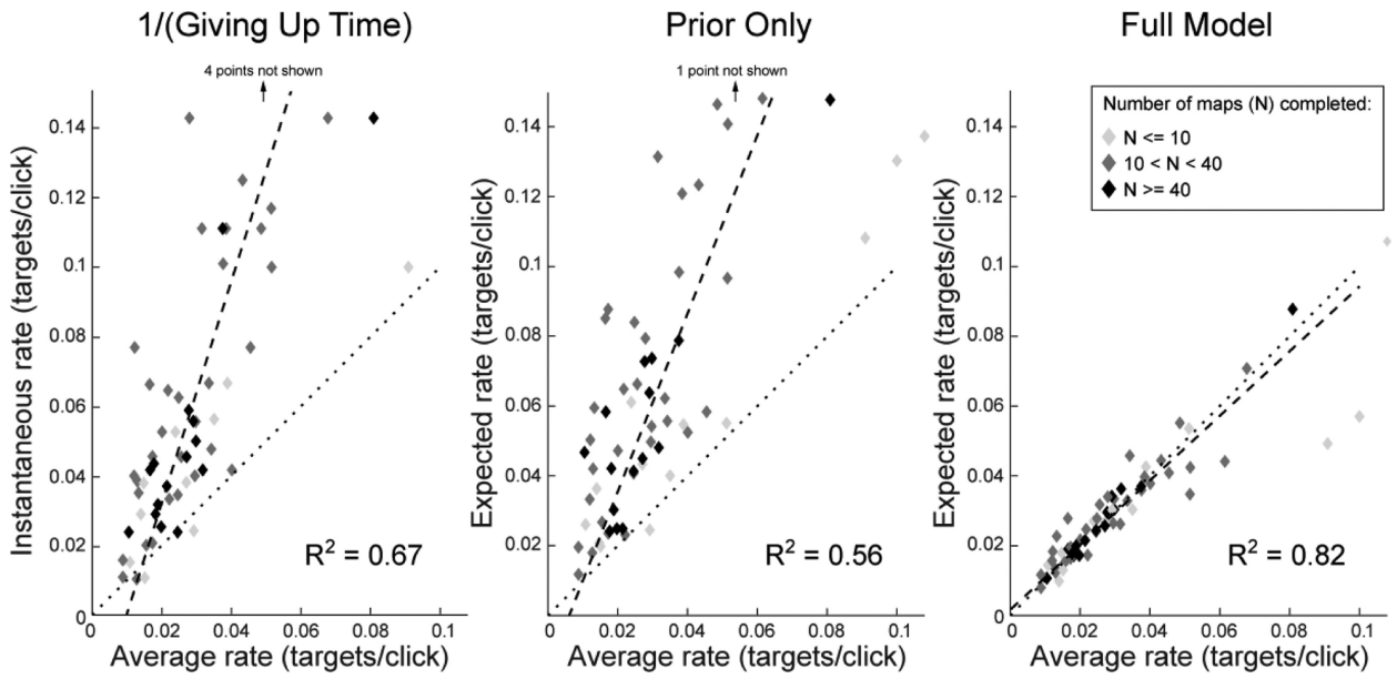
Figure 7. Plots of participants' median rate when quitting trials vs. their average rates in Experiment 1, for various models. Each diamond represents a participant, with color coding the number of maps that participant completed (out of 50). The dotted line indicates the identity (1:1) line: if participants left the patch when their expected rate was exactly the average rate, then all points would lie along this line. Dashed lines are the best linear fit to the data; R 2 for each fit is given on the graph.
