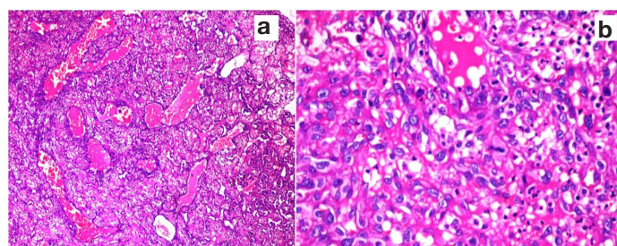
[Table/Fig-3a,b]: a) A photomicrograph showing large areas of distinctive vascular lumens, sometimes anastomosed (H & E, 10x). b) The tumour consisted of spindle to polygonal shaped cells with hyperchromatic nuclei and conspicuous nucleoli with intracytoplasmic vacuoles and mitotic figures are also seen (H & E, 20x).
