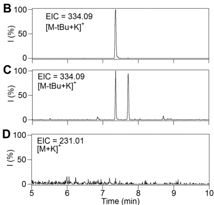
Figure 1. Photolysis reaction of Hc-protected Boc-cysteamine. (A) Structures used in this study. (B) EIC chromatogram ( m/z = 334.09 , calcd for [M(7)-tBu+K]^+ = 334.01 ) of a 50 \mu\text{M} solution of 7 in photolysis buffer (50 mM phosphate buffer, pH 7.4 containing 1 mM DTT) before irradiation, (C) EIC chromatogram ( m/z = 334.09 , calcd for [M(7)-tBu+K]^+ = 334.01 ) of a 50 \mu\text{M} solution of 7 in photolysis buffer after 6 min irradiation at 365 nm, this data clearly indicates generation of the photo-isomer, (D) EIC chromatogram ( m/z = 231.01 , calcd for
