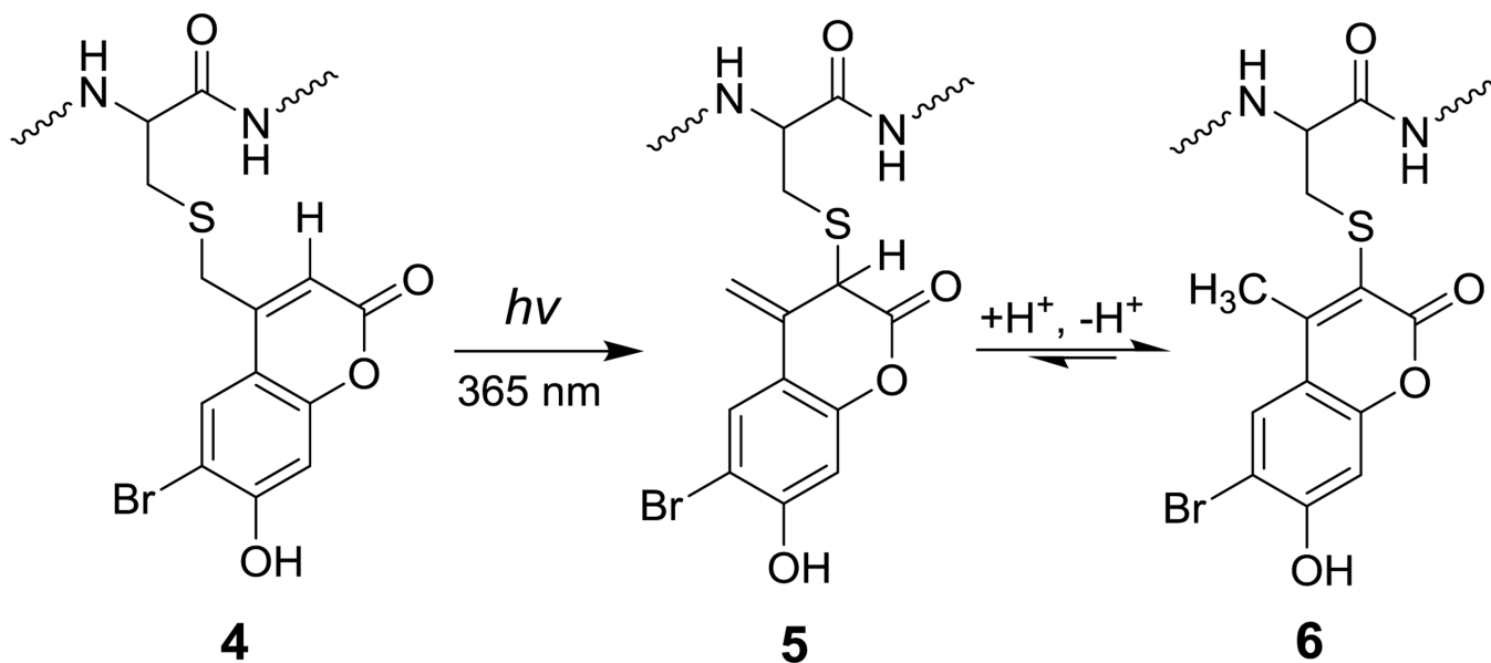
Scheme 2. Photo-rearrangement mechanism of Bhc protected cysteine.
