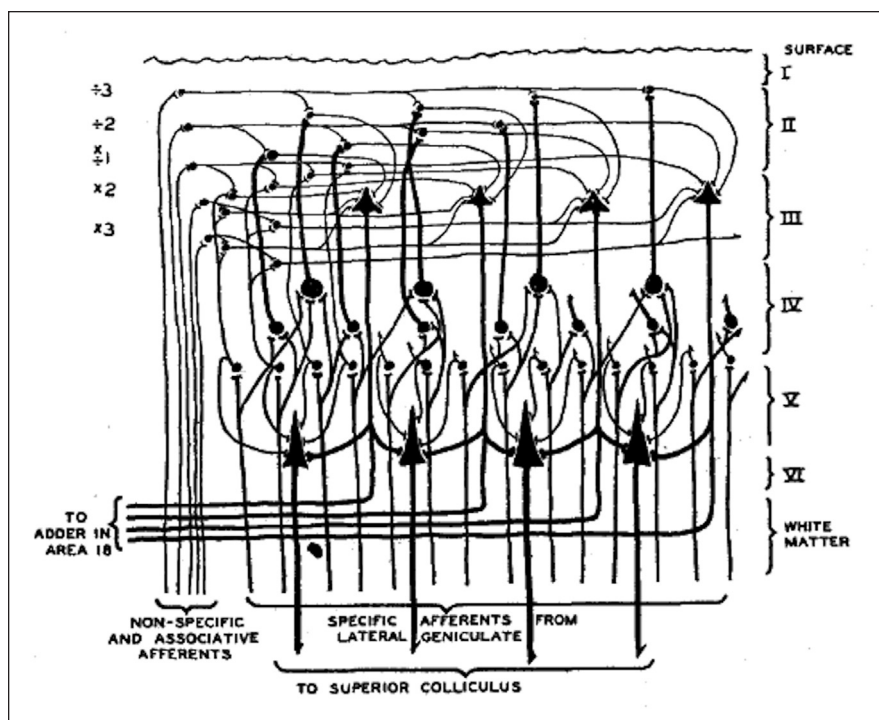
Figure 1: Pitts and McCulloch's model of the visual cortex. Impulses relayed by the lateral geniculate move down to layer IV, where they branch laterally and excite small cells singly and larger cells by summation. Large cells thus represent larger visual areas. From layer IV, impulses go to higher layers. From there, they converge on large cells of the third layer that relay impulses to the parastriate area 18. On their way down, they contribute to summation on the large pyramids of layer V, which relays them to the superior colliculus. Reproduced, with permission of Springer, from "How we know universals: the perception of auditory and visual forms" (W. Pitts and W.S. McCulloch), 6 Bulletin of Mathematics and Biophysics 1947;9:127-47. Copyright © 1947 University of Chicago Press.
