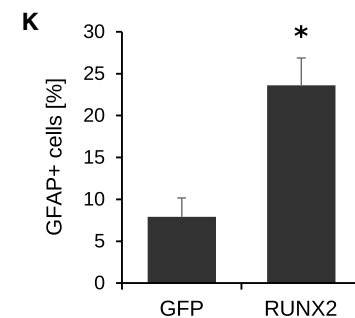
Figure 3. Predicted Opposing Cell-Fate Determinant Pairs, Their GRN Motifs, and Their Experimental Validation in mNSCs
