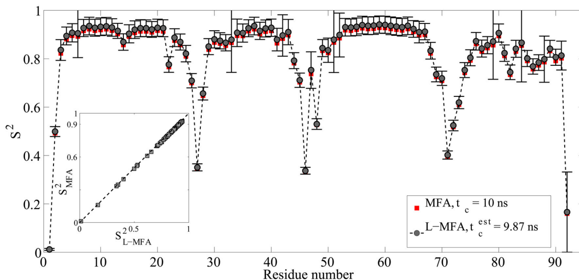
Figure 2. Comparison of backbone N-H S^2 order parameters obtained by L-MFA and MFA model-free analysis of the \alpha -domain of ATPase (PDB 1QZM) based on NMR spin relaxation data computed from a 500 ns MD trajectory assuming a tumbling correlation time \tau_c = 10 ns. An estimated \tau_c = 9.87 ns based on the average R_2/R_1 ratio of residues in well-defined secondary structures was used for the L-MFA analysis. The inset shows a correlation plot of S^2_{MFA} vs. S^2_{L-MFA} with different \tau_c values of 10 and 9.87 ns, respectively. The correlation coefficient between S^2_{MFA} and S^2_{L-MFA} is 1.00 and the RMS error is 0.012.
