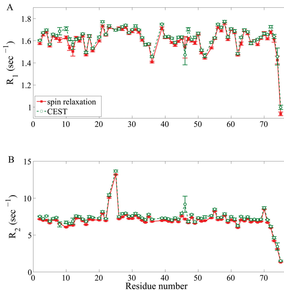
Figure 1. Comparison of experimental relaxation parameters (A) R_1 and (B) R_2 of ubiquitin derived from CEST (green circles) and standard spin relaxation experiments (red squares) at 850 MHz magnetic field strength. Residue T9 is not shown due to substantial broadening of this peak at pH 7 resulting in a large uncertainty of its relaxation parameters.
