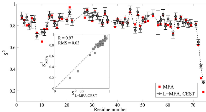
Figure 3. Comparison of experimental ubiquitin order parameters S^2_{MFA} determined from R_1 , R_2 and NOE data of standard spin relaxation experiments (red squares) and S^2_{L-MFA} determined from CEST-derived R_1 , R_2 values (black circles). The insets show scatter plots for the two types of order parameters.
