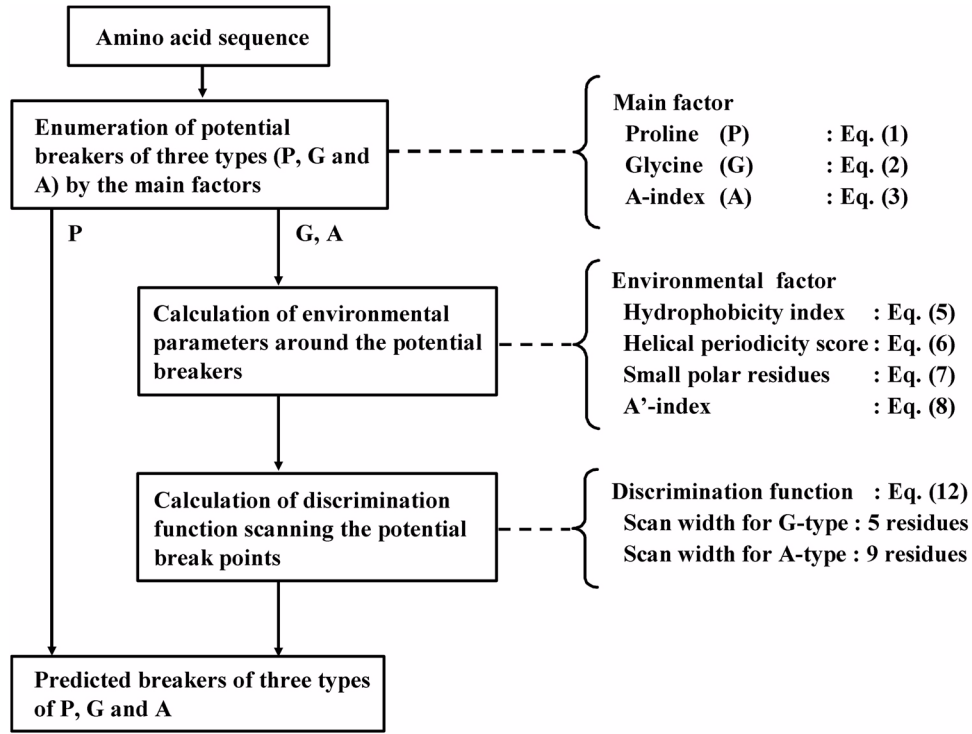
Figure 3 Flow chart of prediction of secondary structure breakers.
