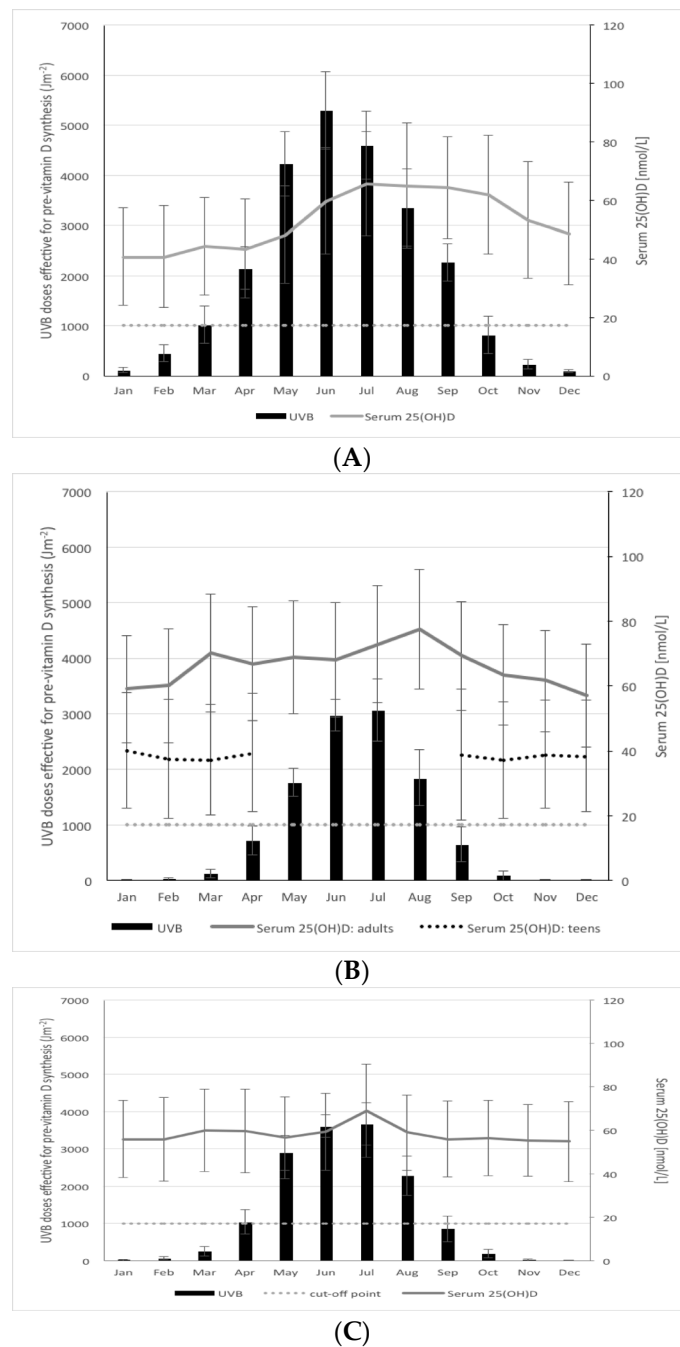
Figure 4. Mean modeled UVB doses effective for pre-vitamin D 3 synthesis ( \text{Jm}^{-2} ) on a monthly basis in a typical year (mean of 2003–2012) in Ireland (51–54° N) and mean (SD) monthly serum 25(OH)D measured in adults (18–84 years) in the National Adult Nutrition Survey in Ireland [21] (A); in Tromsø, Northern Norway (69° N) and mean (SD) monthly serum 25(OH)D measured in adults (18–83 years) in the regionally representative Tromsø sixth cycle cohort [17] (solid line) and adolescents (15–18 years) in the Tromsø—Fit Futures study [18] (dotted black line) (B); and in Reykjavik, Iceland (64° N) and mean (SD) monthly serum 25(OH)D measured in adults (aged 66–96 years) in the regionally representative AGES-Reykjavik cohort in Iceland [19] (C). Note: Data on serum 25(OH)D for the four summer months (May to August) are absent in Tromsø—Fit Futures study as the adolescents were not sampled in this period due to school summer vacation. Dotted line reflects a threshold of 1000 \text{ Jm}^{-2} as a guide to a dose below which dermal synthesis of pre-vitamin D 3 is relatively low. Black bars and error bars represent mean and SD monthly UVB doses, respectively.
