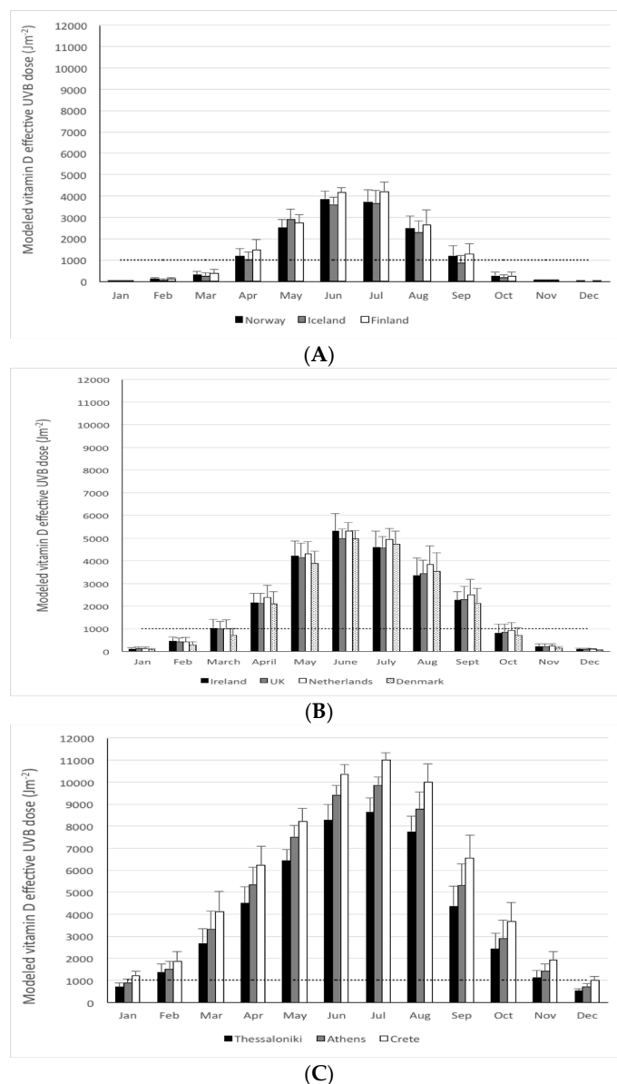
Figure 2. Mean modeled UVB doses effective for pre-vitamin D 3 synthesis ( \text{Jm}^{-2} ) in Norway (mean of Oslo (60° N) and Tromsø (69° N)), Iceland (Reykjavik (64° N)) and Finland (60–70° N) (A); Ireland (51–54° N), the UK (50–59° N), Netherlands (Amsterdam, (52° N)), and Denmark (mean of Copenhagen and Aarhus (56° N)) (B); and Thessaloniki (40° N), Athens (37° N) and Crete (35° N) (C) on a monthly basis in a typical year (mean of 2003–2012). Dotted line reflects a threshold of 1000 \text{ Jm}^{-2} as a guide to a dose below which dermal synthesis of pre-vitamin D 3 is relatively low.
