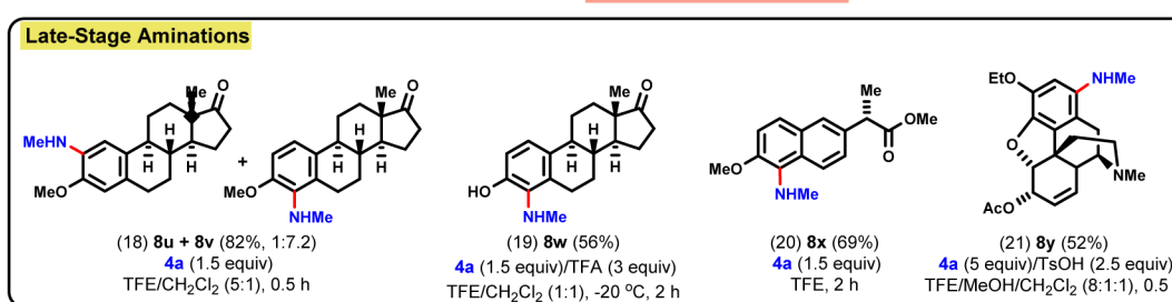
Fig. 2. Direct intermolecular amination of arenes
