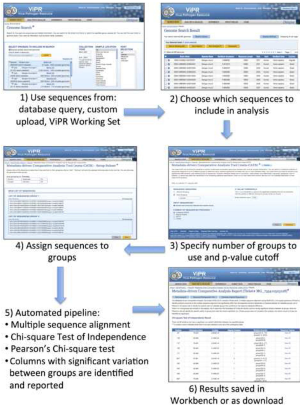
Figure 1. Screenshots of the meta-CATS tool
