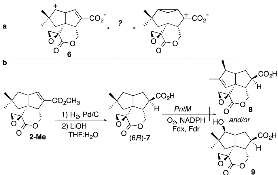
Scheme 3. 6,7-Dihydropentalenolactone F ( 7 )
