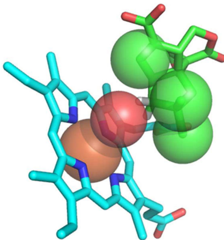
Figure 5. Model showing steric hindrance to oxygen rebound to the C1 si face of pentalenolactone F.
