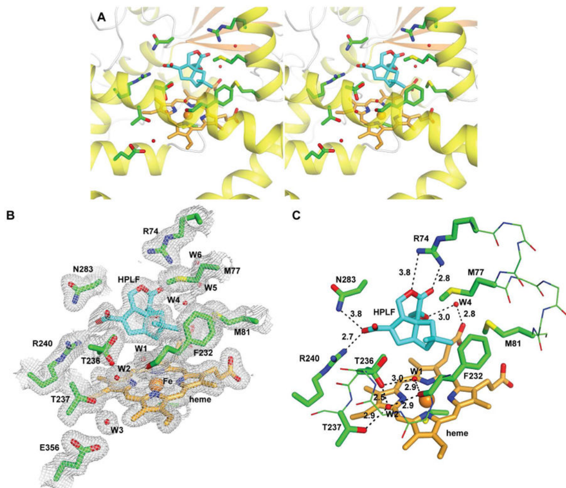
Figure 4. Structure of PntM with bound substrate analogue 7. A, stereo diagram showing heme/analogue 7-binding site. 7 is shown as sticks with carbon atoms in cyan. B, final 2mF_o - DF_c electron density map of the active site region (contoured at 1\sigma ). C, close-up view showing relevant water molecules and H-bonds positioning 7 in the active site.
