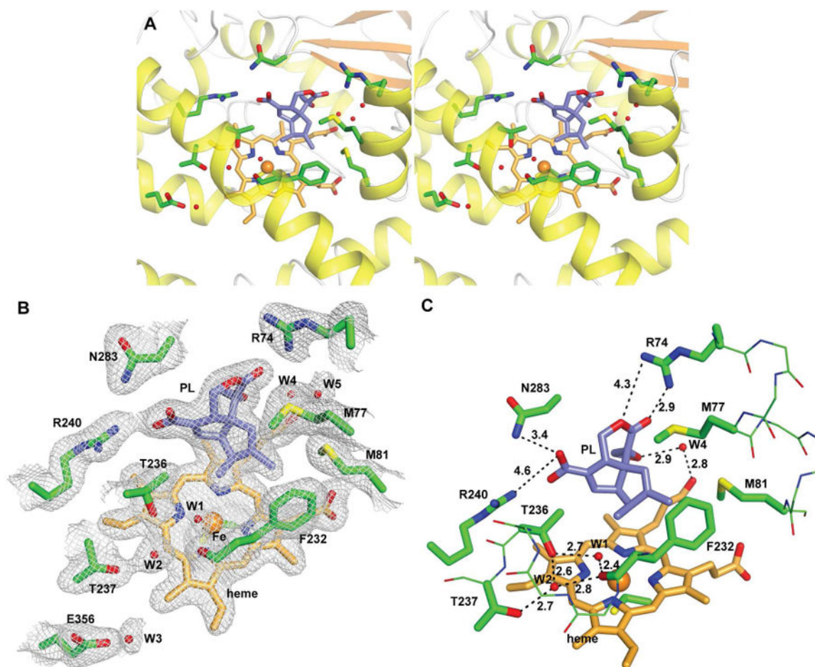
Figure 3. Structure of PntM with bound product 1 . A, stereo diagram showing heme/product 1 -binding site. 1 is shown as sticks with carbon atoms in white/blue. B, final 2mF_o - DF_c electron density map of the active site region (contoured at 1 \sigma ). C, close-up view showing relevant water molecules and H-bonds positioning product 1 in the active site.
