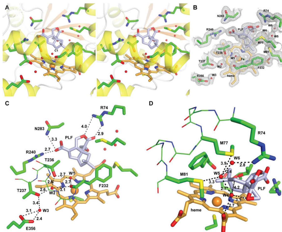
Figure 2. Structure of PntM with bound substrate 2 . A, stereo diagram showing heme/substrate 2 -binding site. 2 is shown as sticks with carbon atoms in light blue. B, final 2mF_0 - DF_c electron density map of the active site region (contoured at 1\sigma ). C, close-up view showing water relay 1 (W1, W2, and W3) and H-bonds positioning substrate 2 . D, close-up view showing water relay 2 (W4, W5, W6).
