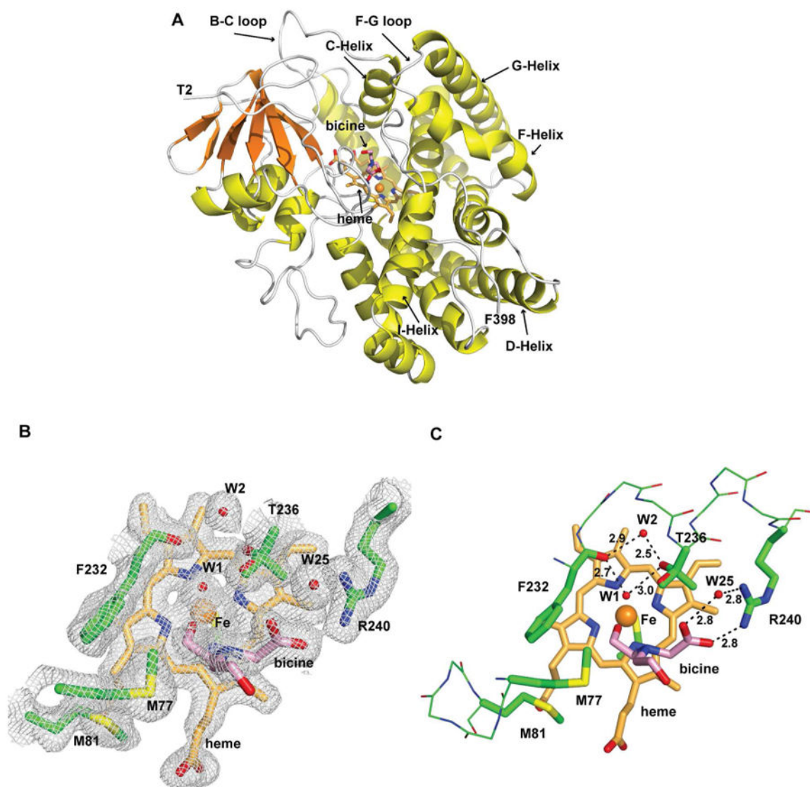
Figure 1. Structure of substrate-free PntM. A, Schematic representation of the structure of PntM with bound bicine. Bicine is shown as sticks with carbon atoms in pink, the heme cofactor is shown as sticks with carbon atoms in bright orange and the heme-bound \text{Fe}^{3+} is shown as an orange sphere. T2 is the N-terminal amino acid and F398 is the C-terminal amino. B, Final 2mF_o - DF_c electron density map of the active site region (contoured at 1 \sigma ). C, close-up view, including relevant water molecules (small red spheres) and H-bonds (distances in Å) that position bicine in the active site.
