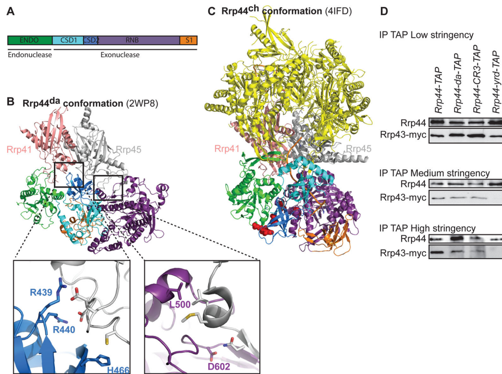
Figure 1. Identification of residues important for the direct access conformation of the RNA exosome
