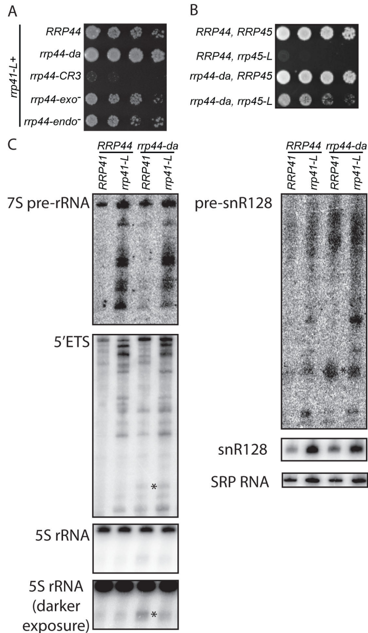
Figure 5. The balance between two RNA exosome conformations is required for growth (A) (B) rrp44-da suppresses the growth defect of rrp41-L and rrp45-L . rrp44 rrp41 or rrp44 rrp45 strains carrying RRP44 variants in a LEU2 plasmid and a wild-type RRP41 or RRP45 in a URA3 plasmid were transformed with a TRP1 plasmid carrying the rrp41-L or rrp45-L allele. Transformants were serially diluted and spotted on 5FOA media. (C) rrp44 rrp41 strains carrying RRP44 and RRP41 variants were subjected to total RNA isolation followed by northern blot analysis probing 7S pre-rRNA, 5'ETS, 5S rRNA, snR128 snoRNA and SRP RNA. Asterisk (*) indicates 5'ETS, 5S and snR128 RNA species specifically and reproducibly detected in the rrp44-da strain.
