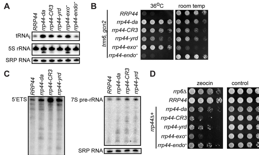
Figure 4. The Rrp44 da -exosome is required for specific functions of the RNA exosome (A) Total RNA isolated from trm6, gcn2, rrp44 strains carrying wild-type or mutant alleles of RRP44 in a LEU2 plasmid were subjected to northern blot. Shown is a representative result of two independent biological replicates. (B) Strains used in (A) were serially diluted and spotted on SC-LEU. (C) Total RNAs were isolated from rrp44 strains carrying a wild-type or mutant RRP44 allele followed by northern blot probing 5'ETS and 7S pre-rRNA. SRP RNA serves a loading control. (D) rrp6 Δ , and rrp44 ΔΔ+ strains carrying wild-type or mutant RRP44 alleles were serially diluted and spotted on media containing 10 μg/ml zeocin and YPD media as a control.
