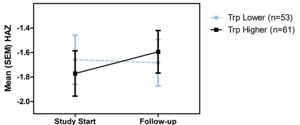
Fig 3. Plasma citrulline (in girls) and tryptophan (in boys) predicts subsequent better growth. A. citrulline (for which gender differs significantly) in girls ( p < 0.001 ; n = 131 ; median citrulline = 23.97 \mu\text{mol/L} ) and B. tryptophan in boys ( p = 0.010 ; n = 114 ; median tryptophan = 66 \mu\text{mol/L} ) predicts subsequent better growth.
