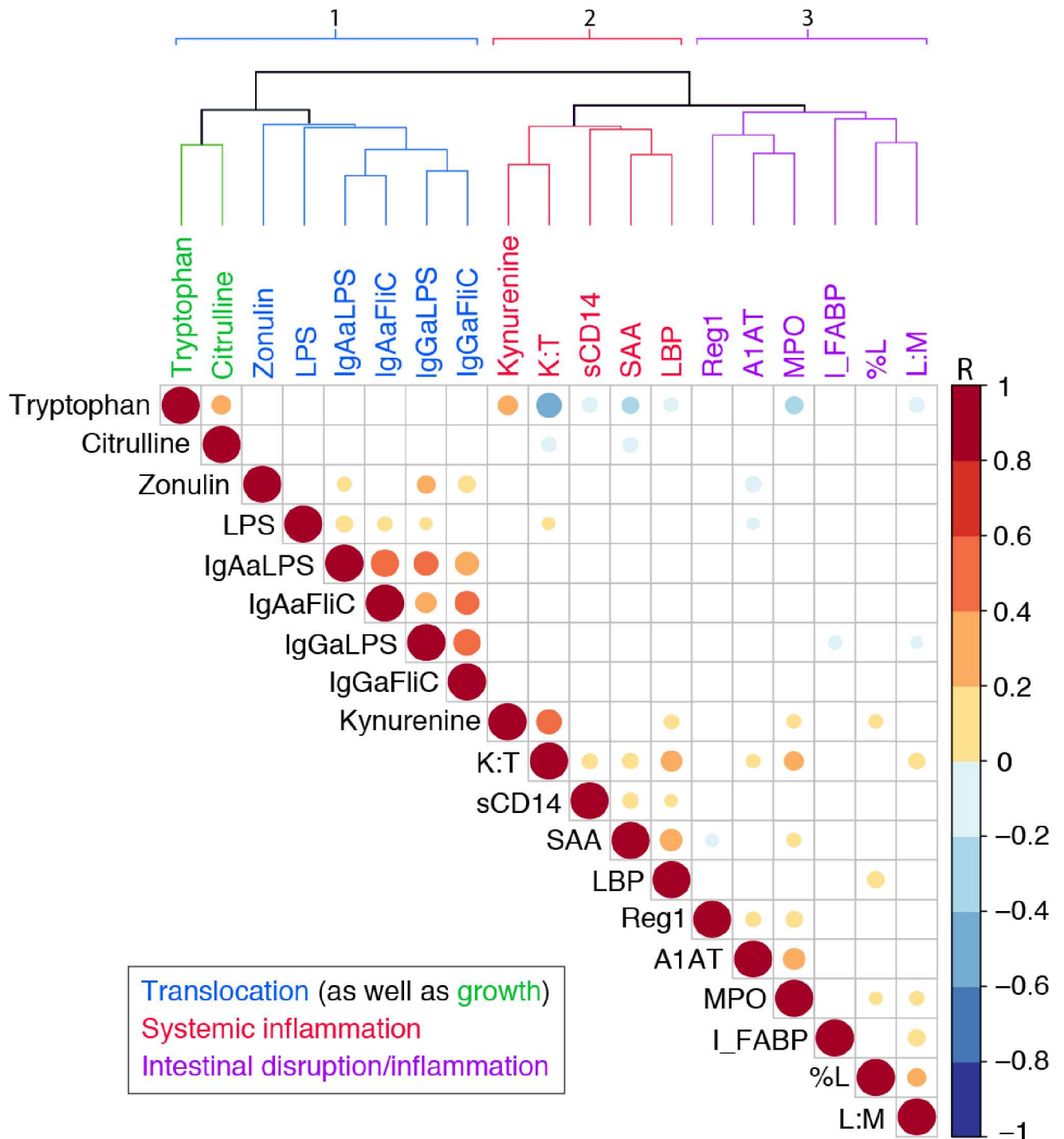
Fig 5. Cluster dendrogram with Pearson correlations among those biomarkers with \geq 274 values showing three main groups: 1) translocation markers, LPS and IgA and IgG anti-LPS or FliC as well as zonulin and the 2 potential predictors of subsequent growth, tryptophan and citrulline; 2) predominantly systemic responses to disrupted barrier function and translocation; and 3) markers of specific intestinal barrier disruption or local intestinal inflammation. As discussed, groups 1 and 3 may predispose to group 2 systemic responses in associating with each other as shown in the heat map as would fit our concept of the pathogenesis of enteropathy.
