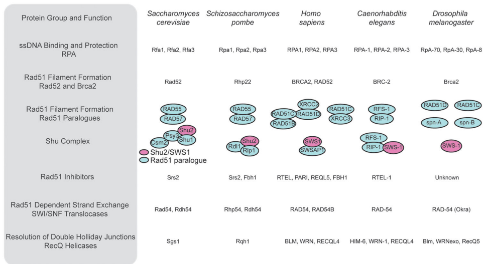
Figure 2. A schematic of the major HR proteins discussed. Homologues in five eukaryotic lineages are shown, and the Rad51 paralogues and the Shu complex, which are discussed in detail in this review, are drawn to show the known complex members in each species.
