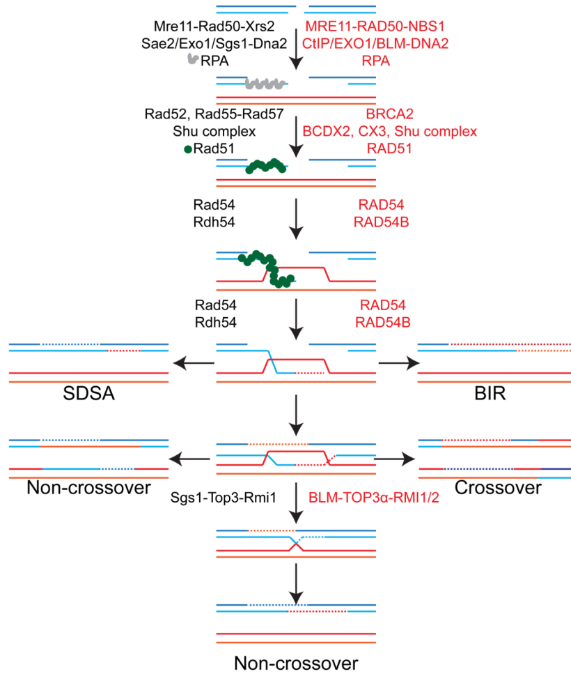
Figure 1. The different pathways utilized during homologous recombination. Protein names in black refer to budding yeast and are used in the legend, while red names refer to human proteins. All pathways begin with recognition of the DSB, followed by resection mediated by the MRX complex in conjunction with Sae2, Exo1, and Sgs1-Dna2 to generate extended 3' ssDNA overhangs. These overhangs are immediately coated by the ssDNA binding protein complex RPA. In order for HR to proceed, Rad51 filaments are induced to form on the ssDNA overhangs by the activity of Rad52, the Rad51 paralogues, and the Shu complex. Rad51 filaments, in conjunction with Rad54 and Rdh54, carry out the critical homology search and strand invasion steps of HR. The strand invasion step is the last common step for all the HR pathways modeled here. During SDSA, the strand invasion product is extended past the break-site before being disassembled and reannealed to the other side of the break, generating a non-crossover repair product. In BIR, the strand invasion product becomes a full replication fork and can progress to the end of the chromosome, creating widespread loss-of-heterozygosity. Alternatively, the second end of the DSB can be captured to generate a double Holliday junction (Center). This double Holliday junction can be cleaved by various nucleases to generate both non-crossover and crossover events as depicted on the left and right respectively. The double Holliday junction can also be dissolved by Sgs1-Top3-Rmi1 to yield non-crossover events. Dashed lines refer to DNA synthesized during HR.
