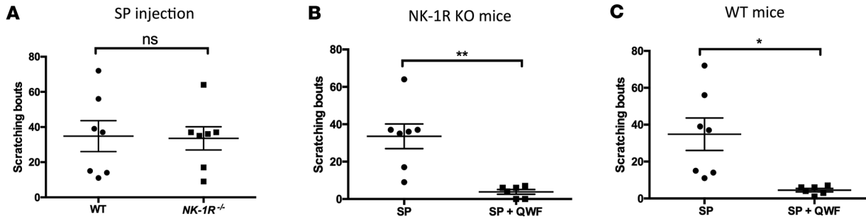
Figure 6. Scratching from substance P is maintained in NK-1R -/- mice and is blocked by QWF. (A) Itch induced by substance P (SP) (500 \mu M) is not decreased in NK-1R -/- mice compared with WT mice. (B) SP-induced itch is significantly decreased ( P = 0.0040 ) in NK-1R -/- mice after coinjection with QWF (500 \mu M). (C) SP-induced itch is significantly decreased ( P = 0.0134 ) in WT mice after coinjection with QWF (500 \mu M). These studies were performed twice using 2-tailed unpaired Student's t test. * P \leq 0.05 , ** P \leq 0.01 .
