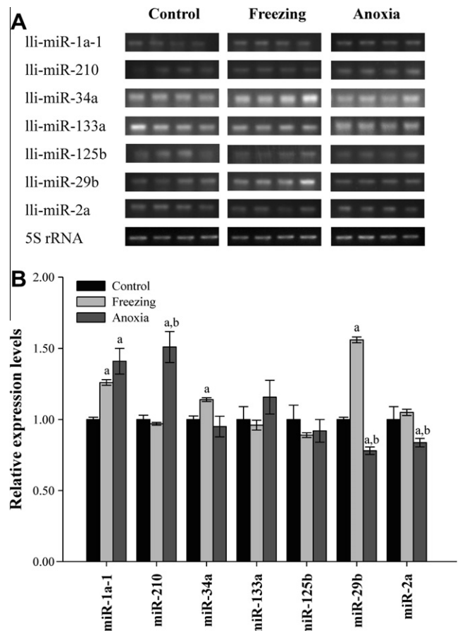
Figure 3 Effect of freezing or anoxia on miRNA expression in the hepatopancreas of L. littorea
