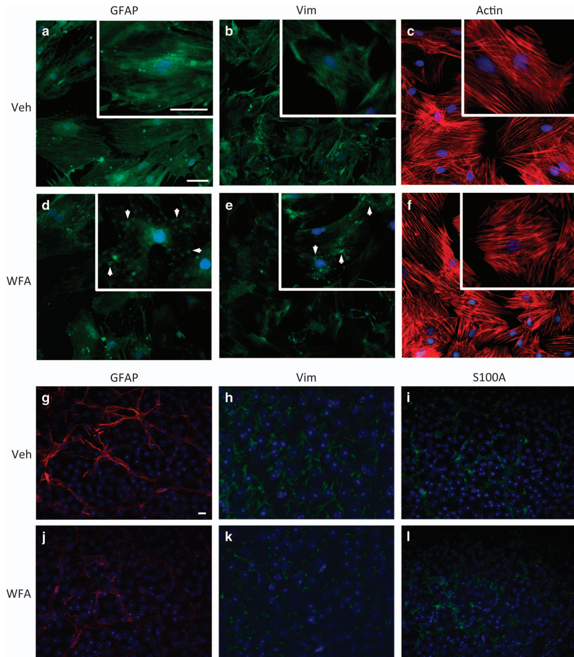
Figure 2 WFA treatment inhibits IF dynamics. (a–f) Treatment of cultured retinal astrocytes with 2.0 \mu\text{m} WFA resulted in reduced staining for GFAP (a and d), and vimentin (vim; b and e), compared with control treated cells after 8 h. At higher magnifications (insets), filamentous staining for GFAP and vimentin was disrupted, resulting in formation of IF aggregates (arrows). In comparison, filamentous actin remained unaffected (c and f). ( n=3 , scale bars indicate 100 \mu\text{m} . Identical exposures were used for all treatments). (g–l) WFA treatment in vivo similarly disrupts GFAP and vimentin in retinal flatmounts, but not S100A. ( n=3 , scale bars indicate 100 \mu\text{m} . Identical exposures were used for all treatments)
