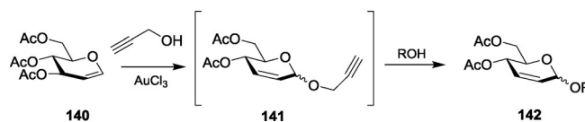
Scheme 32. AuCl 3 -catalyzed propargylation and subsequent glycosylation.
