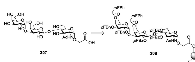
Scheme 44. Solid-phase synthesis of \alpha -Gal trisaccharide epitope.
