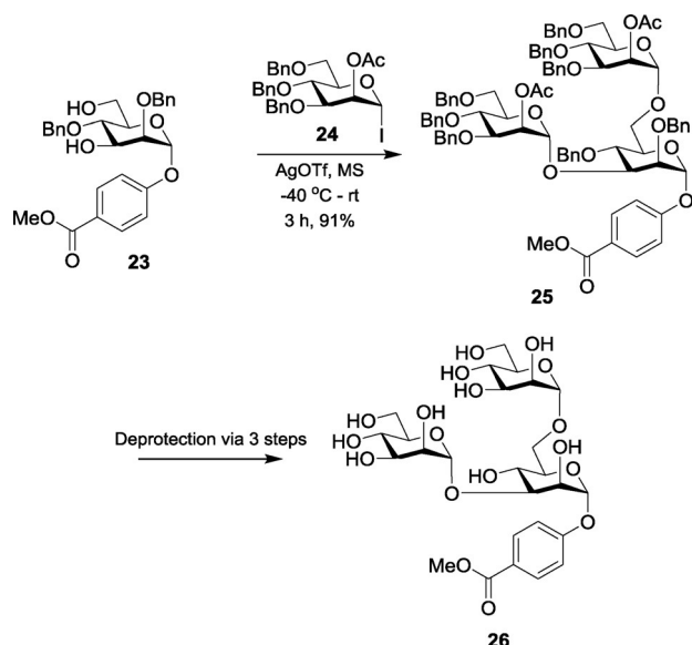
Scheme 5. Synthesis of trimannoside ( 26 ) through double glycosylation.
