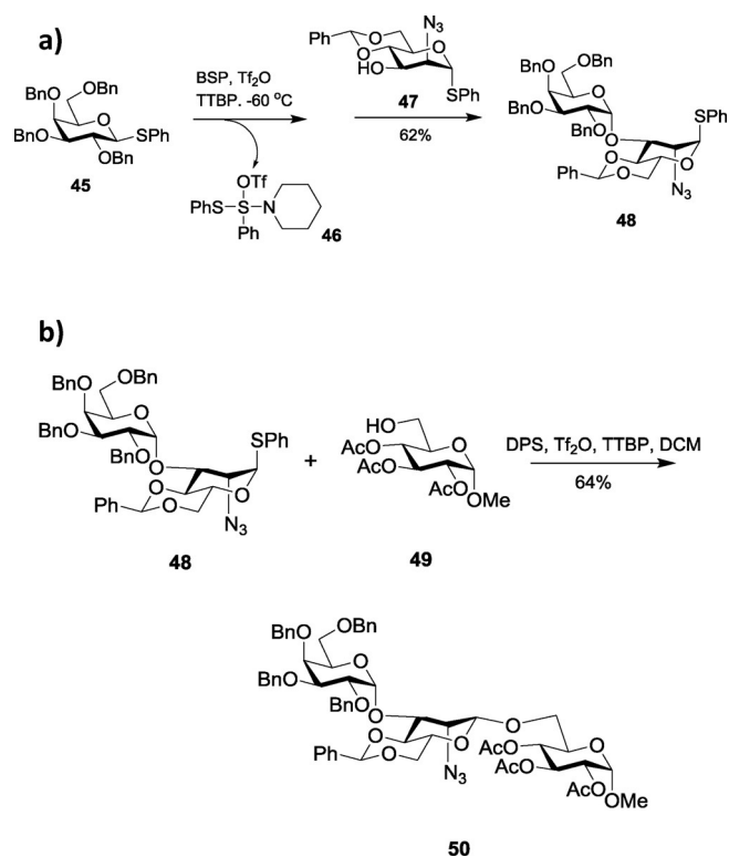
Scheme 11. a) Pre-activation of the donor. b) Subsequent glycosylation with DPS and TTBP as the promoter in the presence of \text{Tf}_2\text{O} .
