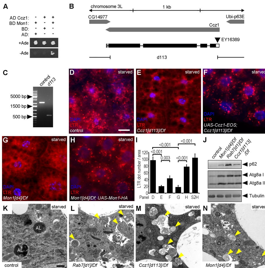
FIGURE 2: Rab7 module mutants are defective in autophagosome-lysosome fusion. (A) Y2H experiment shows the direct interaction of Drosophila Mon1 and Ccz1. (B) Genomic map of the Ccz1 locus. The Ccz1 [d113] allele was generated by imprecise excision of the P-element EY16389. (C) PCR amplification of the Ccz1 locus shows the 1644-base pair deletion in Ccz1 [d113] mutant animals relative to controls. (D–H) Many LTR-positive dots are seen in fat cells of starved control larvae (D). The formation of such acidic compartments is inhibited in Ccz1 (E) and Mon1 (G) mutants and can be restored by expression of wild-type Ccz1 and Mon1 , respectively (F, H). (I) Quantification of LTR data shown in D–H and Supplemental Figure S2H; n = 10 /genotype. (J) Western blots from starved larvae reveal accumulation of the selective autophagic cargo p62 and lipidated, autophagosome-associated Atg8a II in Ccz1 , Mon1 , and Rab7 mutants. Tubulin serves as loading control. (K–N) Electron micrographs of fat cells dissected from starved third-instar larvae. Control cells (K) contain large, electron-dense autolysosomes (AL), whereas Rab7 module mutants (L–N) show accumulation of autophagosomes (arrowheads) and lack of autolysosomes. Scale bar, 20 \mu\text{m} (in D, for D–H), 1 \mu\text{m} (in K, for K–N).
