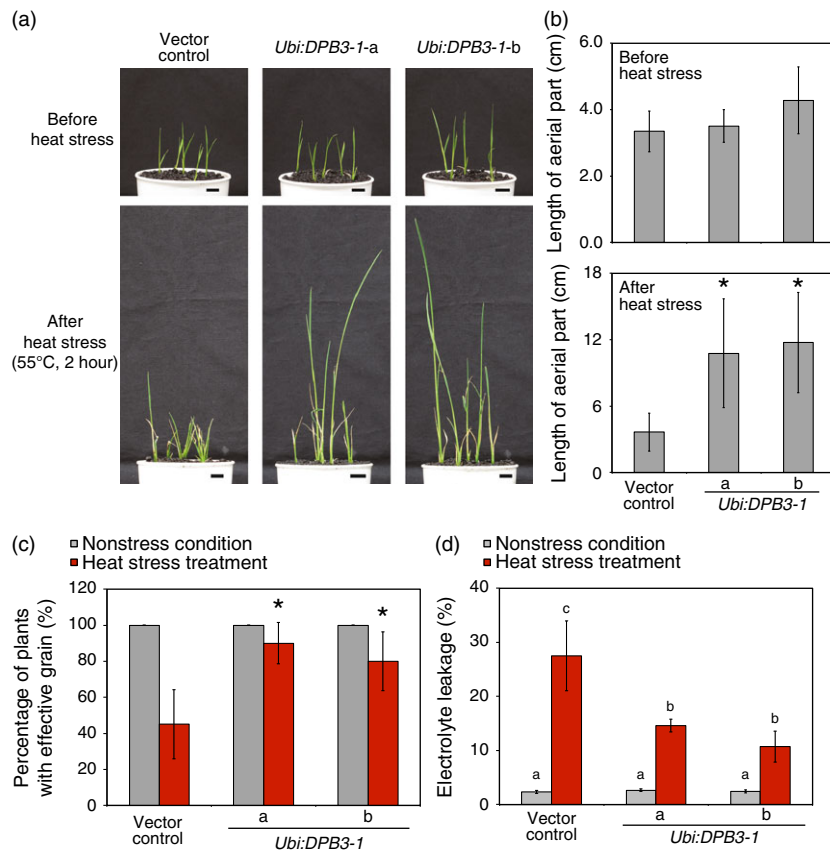
Figure 6 Heat stress tolerance of DPB3-1 -overexpressing plants. (a) Photographs of plants before and after heat stress treatment. The seeds were germinated in water for 7 days at 28 °C, and after germination, the seedlings were grown on soil for 2 days. After heat stress treatment (55 °C, 2 h), the plants were grown under normal conditions. Photographs were taken before stress treatment and after a 10-day recovery period at 28 °C. Scale bars represent 1 cm. (b) Average length of the aerial portion of the vector control and DPB3-1 -overexpressing plants before and after heat stress treatment calculated from the plants grown as shown in (a). The error bars indicate the SD ( n = 15 ). Asterisks indicate significant differences between the plants ( P < 0.05 according to the Bonferroni-corrected Student's t -test). (c) Percentage of plants that grew to the reproductive stage under normal conditions or after heat stress treatment. The stress-treated plants were grown continuously under normal conditions, and the percentages of plants that produced grains were scored. All of the plants without heat stress treatment produced grains. The error bars indicate the SD ( n = 15 ). Asterisks indicate significant differences between the plants after heat stress treatment ( P < 0.05 according to the Bonferroni-corrected Student's t -test). (d) Electrolyte leakage of plants with or without heat stress treatment (42 °C, 24 h). The error bars indicate the SD ( n = 12 ). There were no significant differences between plants without heat stress ( P > 0.05 according to one-way ANOVA), and letters indicate significant differences between the plants after heat stress treatment ( P < 0.05 according to Tukey's multiple range test).
