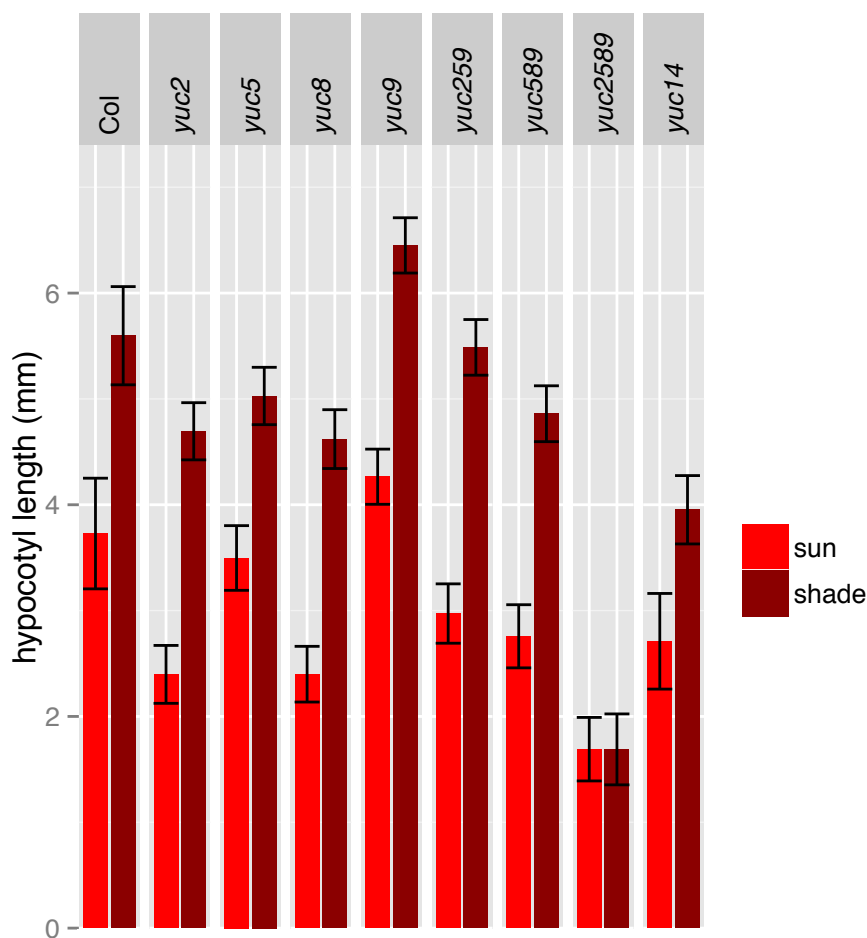
Figure 5 Hypocotyl length of additional lines in simulated sun and shade. Four independent experiments were performed with a total of 35–150 plants per treatment/genotype combination. For growth conditions see “seedling stage high and low R:FR analysis” in Materials and Methods.
