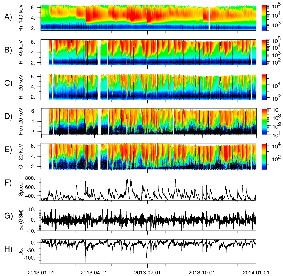
Figure 9. Ion fluxes as a function of L shell and time along with solar wind speed, B_z , and Dst plotted in the same format in Figure 2. (a) 140 keV MagEIS ion measurements. (b) 45 keV HOPE protons. (c–e) 20 keV protons, helium ions, and oxygen ions. Ions with 20 and 45 keV energies penetrate more deeply and decay more quickly than at 140 keV. Comparison with Figures 2 and 7 shows that \sim 140 keV electrons fill the slot quite frequently in 2013 while 140 keV ions were not injected below L \approx 3 .
