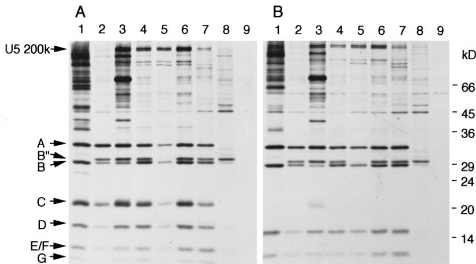
Figure 2. Immunoprecipitation with mAbs to snRNPs. Radiolabeled mouse L929 cell extract was immunoprecipitated with murine mAbs 2.73 (anti-U1-70K, lane 1), 9A9 (anti-U1-A + U2-B''), 22G12 (anti-B'/B, lane 3), Y2 (anti-B'/B and D, lane 4), 2-12 (anti-D, lane 5), 7-13 (anti-D, lane 6), 2G7 (anti-D, lane 7), 4G3 (anti-U2-B''), lane 8), or 162 (anti-Ku antigen, lane 9), and washed with 0.5 M NaCl buffer (panel A) or MMB (panel B).
