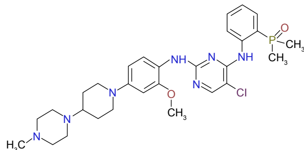
Figure 5 Brigatinib structure.
