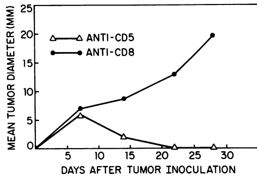
FIG. 4. Effect of anti-CD8 antibody treatment on the tumor growth of mice immunized by N7.2 cells. Groups of five C3H/HeN mice were given an intraperitoneal injection of 5 \times 10^6 N7.2 cells and 1.0 ml of PBS-diluted ascites fluid containing 1 mg of anti-CD8 mAb or, as control, an anti-CD5 mAb. This was followed on the same day by a second injection of 4 \times 10^6 E7C3 cells on the right side of the back of mice.
