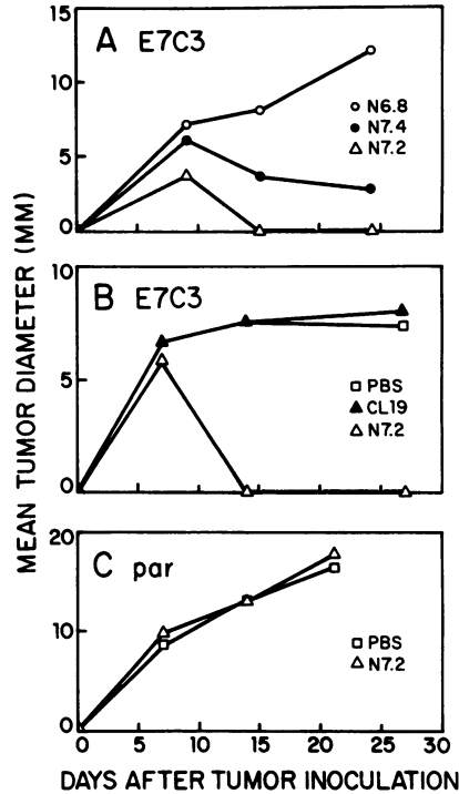
FIG. 3. Growth of murine melanoma cell line E7C3 (par cells transfected with the HPV-16 E7 gene) (A and B) and par cells (E7 negative) (C) in syngeneic C3H/HeN mice immunized with NCTC 2555 fibroblasts that have been transfected with the HPV-16 E7 gene. (A) Groups of five mice were given an intraperitoneal injection of 5 \times 10^6 cells from N6.8 (NCTC2555-derived HPV-16 E6 transfectant) or from either N7.2 or N7.4 (NCTC2555-derived HPV-16 E7 transfectants). (B) Mice were immunized with 5 \times 10^6 N7.2 or CL19 cells (NCTC2555-derived p97 transfectant) or given PBS. In both panels this was followed on the same day by 4 \times 10^6 E7C3 cells transplanted on the right side of the back of mice. (C) Groups of five mice were given an intraperitoneal injection of 5 \times 10^6 N7.2 cells or PBS followed on the same day by 4 \times 10^6 par cells transplanted on the right side of the back of mice.
