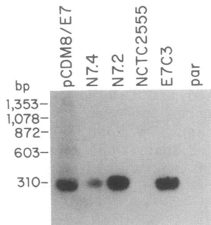
FIG. 2. Southern blot analysis of RT-PCR products from cytoplasmic RNA of HPV-16 E7 transfectants. Lanes: pCDM8/E7, pCDM8/E7 plasmid, amplified by PCR as a positive control; N7.4 and N7.2, NCTC2555-derived HPV-16 E7 transfectants; NCTC2555, the negative control; E7C3, par-derived HPV-16 E7 transfectant; par, negative control. Transfectant mRNA (1 µg) was used in the RT-PCR and 1 ng of pCDM8/E7 plasmid was used in the PCR. bp, Base pairs.
