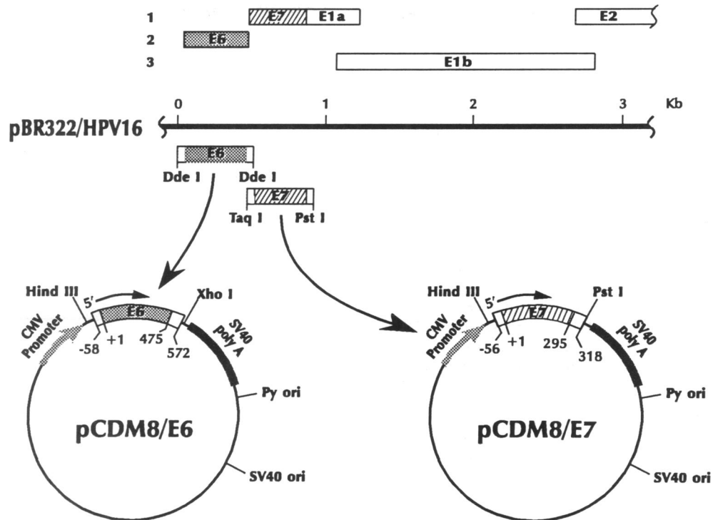
FIG. 1. Construction of the HPV-16 E7 -expressing plasmid pCDM8/ E7 and the E6 -expressing plasmid pCDM8/ E6 . The entire HPV-16 E7 or E6 ORF was inserted into the Hind III- Pst I or Hind III- Xho I sites, respectively, of pCDM8 plasmids downstream of the cytomegalovirus (CMV) promoter and upstream of the SV40 poly(A) + signal. The figure is not drawn to scale. kb, Kilobase(s).
