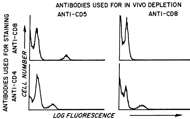
FIG. 5. Flow cytometry analysis of splenocytes from mice treated with anti-CD8 mAb (Right) or mice treated with anti-CD5 mAb (Left). The antibodies were administered intraperitoneally as described in Fig. 4. Spleens were removed at day 21 after antibody treatment, and single-cell suspensions were obtained. (Left) Staining profiles of control group splenocytes using fluorescein isothiocyanate-conjugated anti-CD8 and anti-CD4 antibodies. (Right) Staining profiles of splenocytes from anti-CD8-depleted mice are shown. A total of 10^4 cells was analyzed in each panel.
