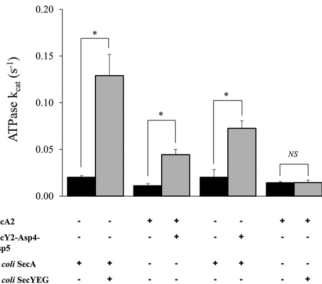
FIGURE 6. ATPase activities of S. gordonii SecA2 with and without SecY2-Asp4-Asp5. Steady-state ATPase activity of 0.3 \mu M S. gordonii SecA2 or E. coli SecA in the presence of 0.46 \mu M S. gordonii SecY2-Asp4-Asp5 or E. coli SecYEG, reconstituted in proteoliposomes. Statistical significance is indicated by an asterisk (*, p < 0.05 , t test). No statistical significance (NS) is also indicated. Error bars are \pm S.E. ( n = 5 ).
