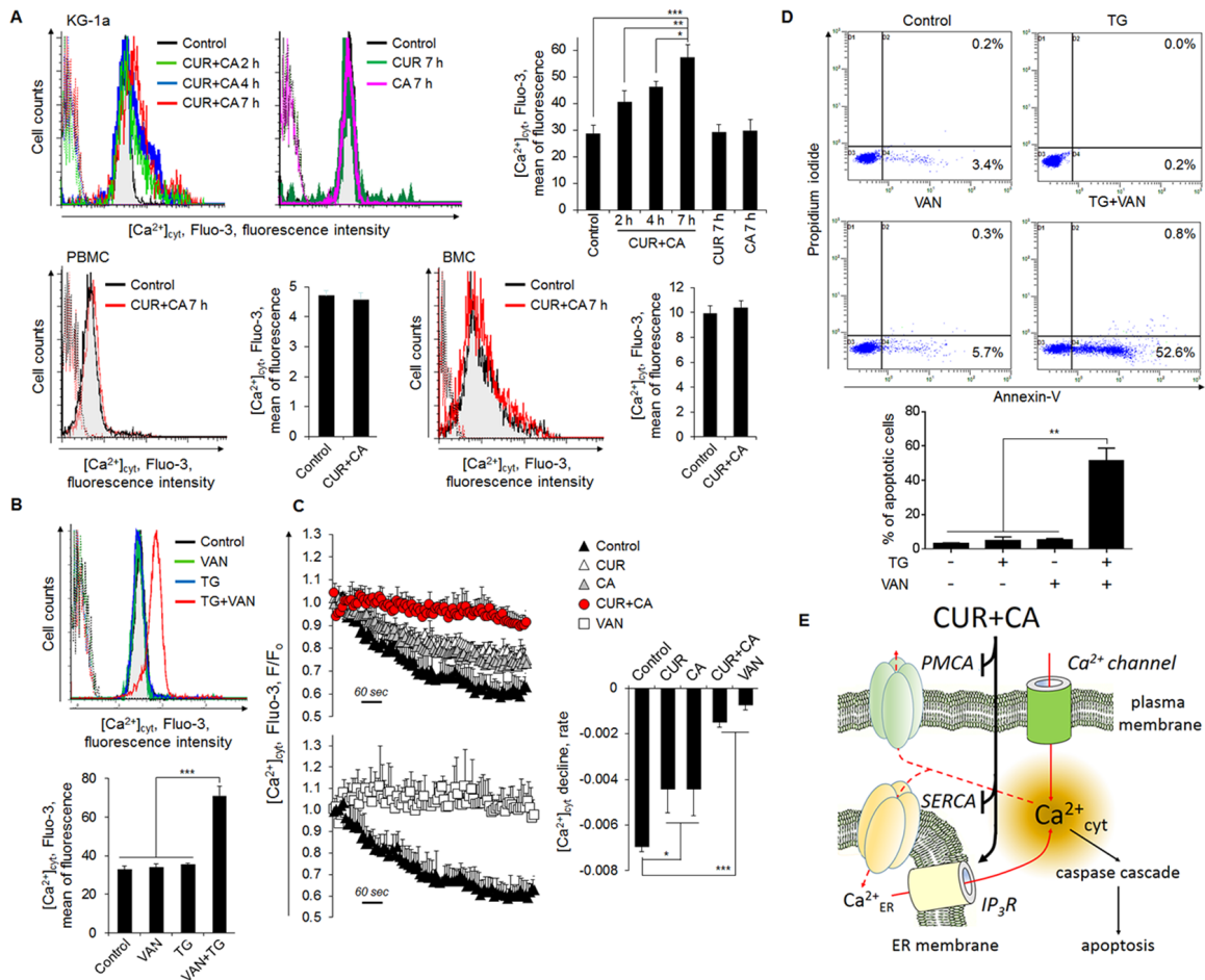
Figure 6: Compromised extrusion of \text{Ca}^{2+} through the plasma membrane contributes to sustained \text{Ca}^{2+}_{\text{cyt}} rise in CUR+CA-treated AML cells and, thereby, to apoptosis. (A) CUR+CA treatment elevates steady-state \text{Ca}^{2+}_{\text{cyt}} levels in KG-1a cells but not in PBMC or BMC. [\text{Ca}^{2+}]_{\text{cyt}} is expressed as the mean Fluo-3 fluorescence intensity measured by flow cytometry. Presented are histogram overlays from a typical experiment showing [\text{Ca}^{2+}]_{\text{cyt}} at the indicated time points of CUR+CA treatment. Overlapping dotted curves in the first logarithmic decade depict autofluorescence. Bar graphs show averaged mean Fluo-3 fluorescence intensities \pm SD measured in a representative of 3 independent experiments performed in triplicate. (B) [\text{Ca}^{2+}]_{\text{cyt}} was assessed in KG-1a cells treated with thapsigargin (TG; 200 nM) and/or the PMCA blocker sodium orthovanadate (VAN; 1 mM) for 7 h, as described in (A). (C) CUR+CA treatment blocks \text{Ca}^{2+}_{\text{cyt}} extrusion through the plasma membrane. Fluo-3-labeled KG-1a cells were loaded with \text{Ca}^{2+} and extrusion of \text{Ca}^{2+}_{\text{cyt}} was assessed by flow cytometry as the time-dependent decline in Fluo-3 fluorescence, as described in Materials and Methods . VAN was used as a positive control for inhibition of plasma membrane \text{Ca}^{2+} efflux. Curves show means \pm SD of F/F 0 ratios from a representative of 3 experiments performed in triplicate. Bar graphs show mean F/F 0 ratios \pm SD. (D) Modeling of CUR+CA-induced apoptosis by combined treatment of KG-1a cells with TG (200 nM) and VAN (1 mM) for 7 h. Apoptosis was assessed by the annexin-V/PI binding assay. Upper panel : typical dot plots from a representative of 3 independent experiments. Lower panel : averaged percentages of apoptotic (early+late) cells measured in 3 independent experiments (means \pm SD). (E) A pictorial view for the proposed mechanism of CUR+CA-induced apoptotic \text{Ca}^{2+}_{\text{cyt}} overload in AML cells. Low resting [\text{Ca}^{2+}]_{\text{cyt}} is maintained through the action of SERCA and PMCA. By mobilizing \text{Ca}^{2+}_{\text{ER}} (most probably, via the blockade of SERCA and stimulation of \text{IP}_3\text{R} ) and inhibiting PMCA, the CUR+CA combination robustly elevates \text{Ca}^{2+}_{\text{cyt}} levels that triggers caspase-dependent apoptosis. * ( p < 0.05 ), ** ( p < 0.01 ), *** ( p < 0.001 ); Student's t test.
