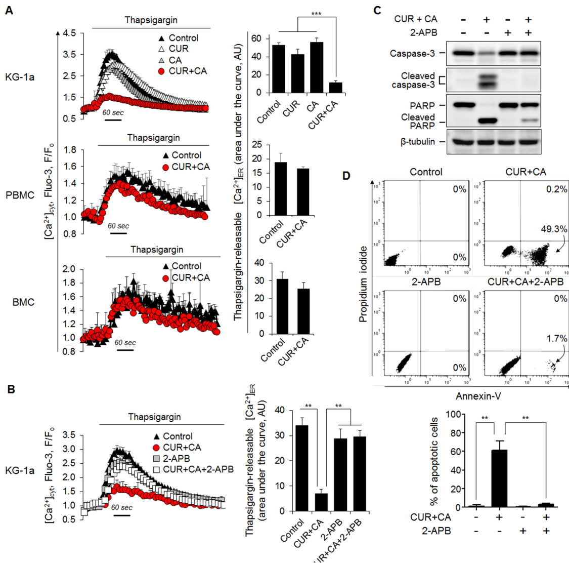
Figure 4: CUR+CA-induced apoptosis is mediated by mobilization of \text{Ca}^{2+} from the ER. (A) CUR+CA treatment depletes thapsigargin-sensitive ER \text{Ca}^{2+} stores in AML cells, but not in non-neoplastic hematopoietic cells. Left panel: Flow cytometric monitoring of [\text{Ca}^{2+}]_{\text{cyt}} in thapsigargin (1 \mu\text{M} )-stimulated Fluo-3-loaded KG-1a, PBMC and BMC cells following treatment with or without CUR+CA for 2 h. Instantaneous changes in Fluo-3 fluorescence (F) were normalized to the resting values ( F_0 ). Curves show means \pm SD of F/ F_0 ratios measured in a typical experiment. Right panel: The extent of thapsigargin-induced \text{Ca}^{2+}_{\text{ER}} release expressed as an area under the curve depicting transient [\text{Ca}^{2+}]_{\text{cyt}} rise followed by [\text{Ca}^{2+}]_{\text{cyt}} decline toward the baseline. The data are the means \pm SD from a representative of 3 experiments performed in triplicate. (B) Depletion of ER \text{Ca}^{2+} stores in CUR+CA-treated KG-1a cells is prevented by the IP3R blocker 2-APB (25 \mu\text{M} ). Left and right panels show means \pm SD of [\text{Ca}^{2+}]_{\text{cyt}} and the extent of thapsigargin-induced \text{Ca}^{2+}_{\text{ER}} release, respectively, measured in a representative of 3 experiments performed in triplicate. (C) Western blot analysis of caspase-3 and PARP cleavage in control and CUR+CA-treated KG-1a cells (7 h) in the presence or absence of 2-APB (25 \mu\text{M} ). (D) Annexin V/propidium iodide assay was used to assess the extent of apoptosis in control and CUR+CA-treated (7 h) KG-1a cells in the presence or absence of 2-APB. Upper panel: dot plots from a typical experiment. Lower panel: averaged percentages of apoptotic (early+late) cells measured in 3 independent experiments performed in triplicate (means \pm SD). **( p < 0.01 ), ***( p < 0.001 ); Student's t test.
