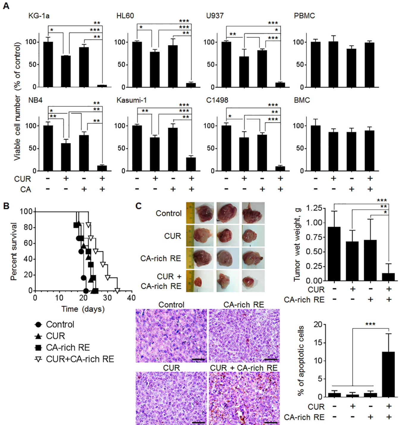
Figure 1: CUR and CA synergistically reduce the numbers of viable AML cells in culture and retard AML development in murine models. (A) Indicated AML and non-neoplastic hematopoietic cell types were treated with 5 \mu M CUR and/or 10 \mu M CA for 72 h. Viable cell numbers were determined by the trypan blue exclusion assay. The data are the means \pm SD from 3–6 independent experiments performed in triplicate. (B) C57BL/6 mice were inoculated i.v. with 5 \times 10^4 C1498 cells. Seven days thereafter, mice were divided into 4 groups of 6 animals and fed with diets containing vehicle (2.05% methylcellulose, w/w), CUR (0.05%, w/w), CA-rich RE (2%, w/w) or CUR+CA-rich RE. Animal survival was estimated by the Kaplan-Meier analysis. (C) SCID/Beige mice were inoculated i.p. with 5 \times 10^6 HL60 cells. Seven days thereafter, mice were divided into 4 groups of 6 animals and treated i.p. with vehicle (0.1% DMSO/PBS), CUR (25 mg/kg), CA-rich RE (25 mg/kg) or CUR+CA-rich RE, 3 times a week for 12 days. Upper left panel : typical tumors excised from control and treated animals. Upper right panel : Averaged tumor weights (means \pm SD) in the indicated groups of mice. * ( p < 0.05 ), ** ( p < 0.01 ), *** ( p < 0.001 ); Student's t test. Lower left panel : TUNEL staining of apoptosis (400 \times ). Scale bars indicate 50 \mu m. Lower right panel : Average percentages of apoptotic cells calculated as described in Materials and Methods. *** ( p < 0.001 ); Student's t test.
