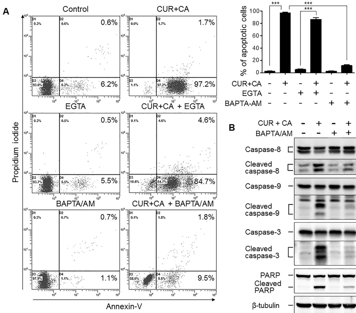
Figure 3: Intracellular but not extracellular \text{Ca}^{2+} mediates the CUR+CA-induced apoptosis in AML cells. (A) Annexin V/propidium iodide assay was used to assess the extent of apoptosis in control and CUR+CA-treated (7 h) KG-1a cells, in the presence or absence of EGTA (1 mM) or BAPTA/AM (2 \mu\text{M} ). Left panel : typical dot plots obtained in a representative experiment. Right panel : averaged percentages of apoptotic (early+late) cells measured in 3 independent experiments (means \pm SD). (B) Western blot analysis of caspase (8, 9 and 3) and PARP cleavage in control and CUR+CA-treated KG-1a cells (7 h), in the presence or absence of BAPTA/AM (2 \mu\text{M} ). ***( p < 0.001 ); Student's t test.
