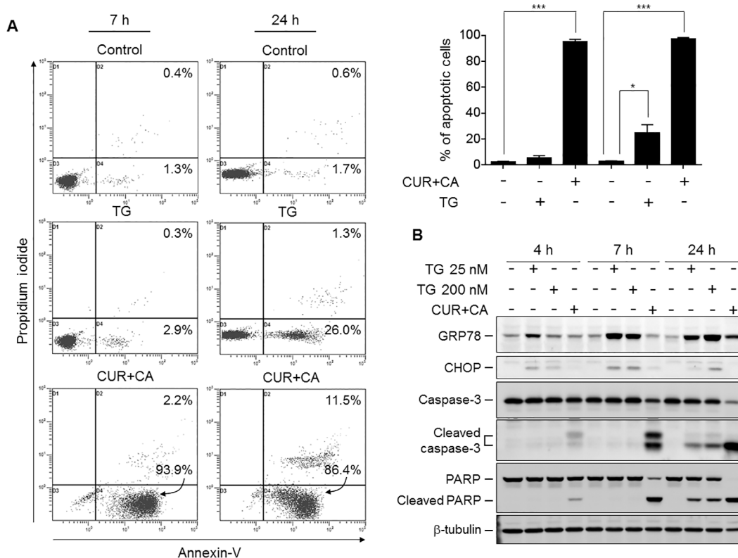
Figure 5: CUR+CA-induced apoptosis is not dependent solely on mobilization of \text{Ca}^{2+}_{\text{ER}} and does not involve ER stress. (A) Comparison of thapsigargin (200 nM)- and CUR+CA-induced apoptosis in KG-1a cells at the indicated time points using the annexin V/propidium iodide binding assay. Upper panel : dot plots from a typical experiment. Lower panel : averaged percentages of apoptotic (early+late) cells measured in 3 independent experiments (means \pm SD). (B) Western blot analysis of the expression of ER stress markers (GRP78; CHOP) and caspase-3 and PARP cleavage in the course of thapsigargin and CUR+CA treatment of KG-1a cells. *( p < 0.05 ), ***( p < 0.001 ); Student's t test.
