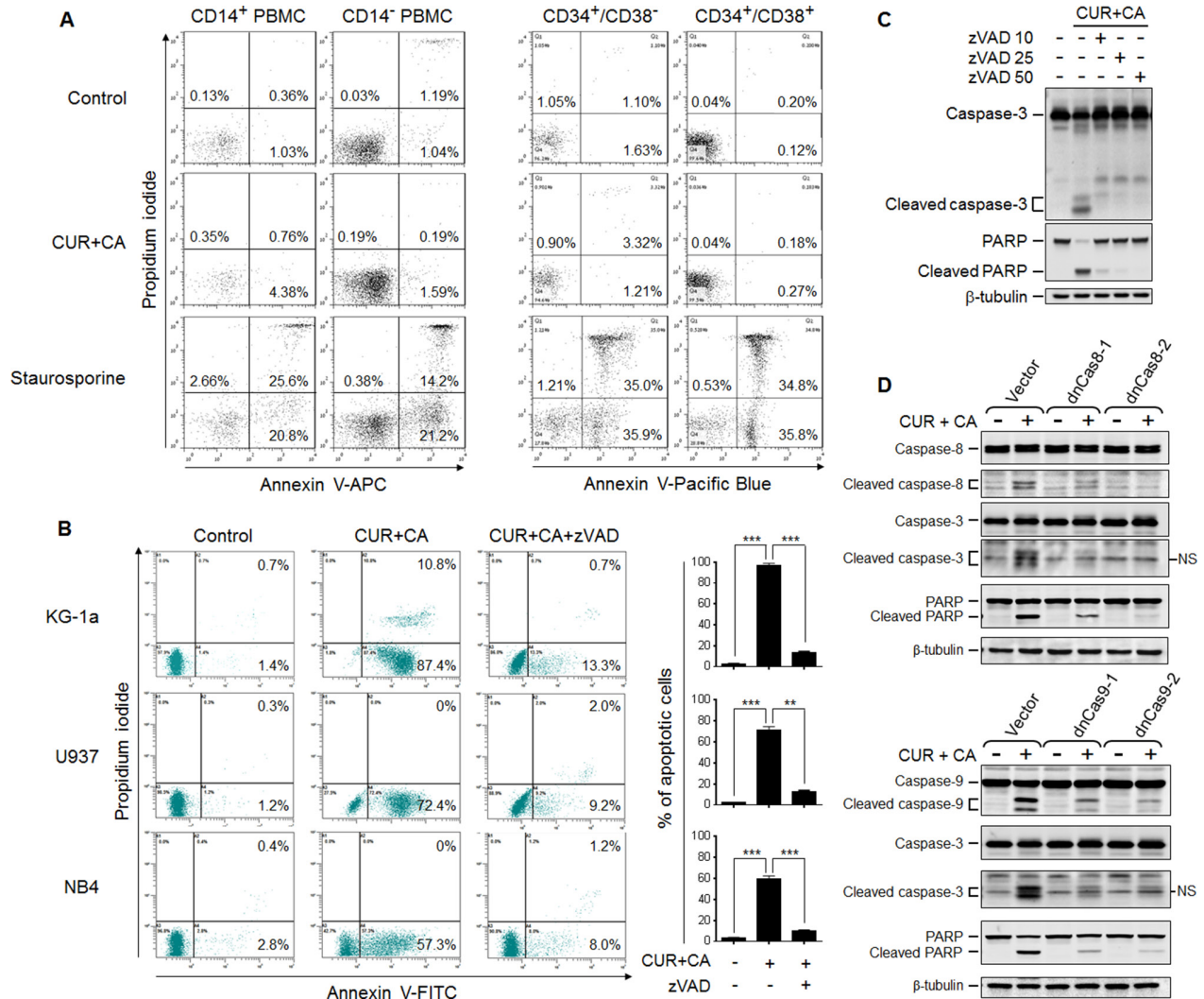
Figure 2: CUR+CA combination induces caspase-dependent apoptosis in AML cells but not in non-neoplastic hematopoietic cells. (A) PBMC (left panel) and umbilical cord blood mononuclear cells (right panel) were treated with vehicle (control) or the CUR+CA combination for 18 h, or with 1.25 \mu M staurosporine (positive control) for 6 h. The extent of apoptosis was determined in the indicated cell populations (Supplementary Figure S2) by flow cytometry using the annexin V/propidium iodide binding assay. Representative panels from at least 3 similar experiments performed in each cell type are shown. (B) Indicated AML cell types were treated with the CUR+CA combination and analyzed for apoptotic responses, as above. Note that apoptosis was nearly abolished by the pan-caspase inhibitor zVAD (50 \mu M). Left panels: typical dot plots obtained in a representative experiment. Percentages of early (annexin V-positive, propidium iodide-negative) and late (annexin V- and propidium iodide-positive) cells are shown. Right panels: percentages of apoptotic (early+late) cells measured in 3 independent experiments (means \pm SD). (C) Western blot analysis of caspase-3 and PARP cleavage in KG-1a cells treated with CUR+CA for 7 h in the presence or absence of zVAD. (D) Caspase (8, 9 and 3) and PARP cleavage in KG-1a cells stably transfected with the empty vector, the dominant-negative caspase-8- (dnCas8; upper panel) or caspase-9- (dnCas9; lower panel) encoding plasmids. Cells were treated with or without CUR+CA for 7 h. Two clones of each dnCas8 and dnCas9 transfectant were used. Data from a representative experiment of 3 performed are shown. **( p < 0.01 ), ***( p < 0.001 ); Student's t test.
