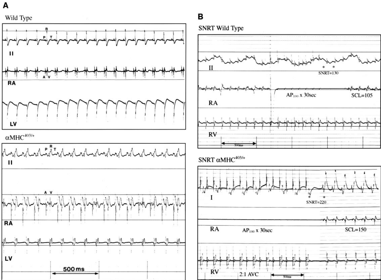
Figure 2. (A) Three-channel recordings during normal sinus rhythm from wild-type (top) and \alpha MHC 403/+ mice (bottom). The surface ECG lead II and intracardiac bipolar electrograms from right atrium (RA) and left ventricle (LV) are shown. On the surface lead, P, R, and T waves are marked during one cardiac cycle. On the atrial electrogram, both an atrial (A) and ventricular (V) deflection are inscribed. The electrograms from the \alpha MHC 403/+ mouse are notable for being markedly fractionated. Paper speed is 100 mm/s, vertical calibration lines are 100 ms markers and horizontal lines are one cm apart (ECG display amplification = 0.1 mV/cm). Surface ECG filters were set between 1 and 50 Hz, and intracardiac electrogram filters were set between 10 and 250 Hz. (B) Sinus node recovery time (SNRT) from wild-type (top) and \alpha MHC 403/+ (bottom) mice. A surface ECG lead and intracardiac right atrial (RA) and right ventricular (RV) bipolar electrograms are displayed. A time break was introduced in the figure during the 30 s of atrial pacing to allow both pacing and SNRT to be shown on the same figure. After 30 s of rapid atrial pacing at 100 ms (AP 100 ), the SNRT is measured from the last paced atrial beat (first asterisk) to the first sinus return beat (second asterisk), corrected for the sinus cycle length (SCL). In the wild-type, the corrected sinus node recovery time (CSNRT = SNRT - SCL) is 130 - 105 = 25 ms. In the \alpha MHC 403/+ mouse, during rapid atrial pacing at 100 ms (AP 100 ), there is 2:1 atrioventricular conduction (2:1 AVC) demonstrated on both the surface ECG and RV electrogram, and following atrial pacing, the CSNRT = 220 - 150 = 70 ms.
