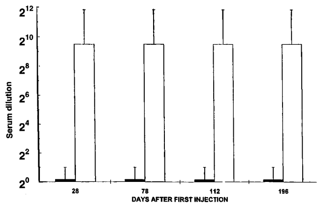
Figure 5. Antiadenovirus neutralizing antibodies levels in group A tolerized (solid bars) and group C control rats (open bars), after the first and second Ad-hBUGT 1 injections. Mean levels were calculated from levels in antibody producing rats.
