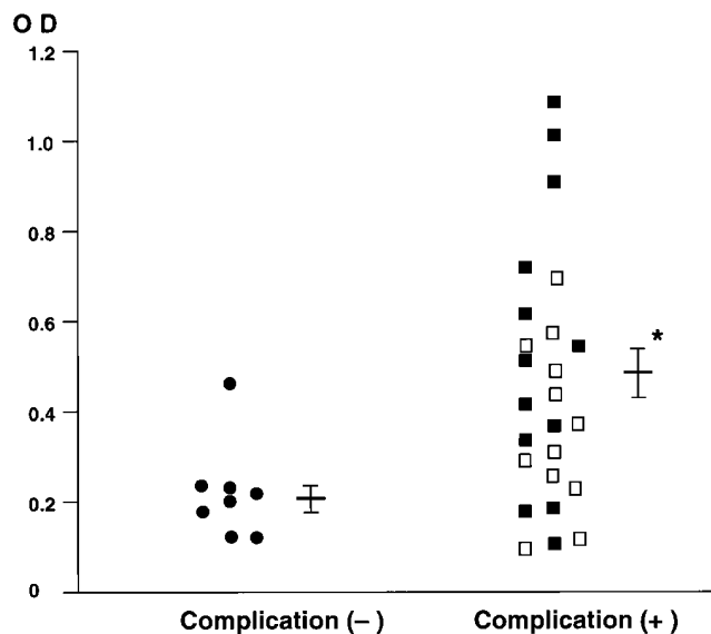
Figure 2. Higher anti-YPM titers among the patients with systemic complications. The patients with Y. pseudotuberculosis infection were classified by the presence ( \blacksquare for IVGG untreated and \square for IVGG treated) or the absence ( \bullet ) of the systemic complications (renal dysfunction, acute abdomen, arthritis, lymphadenopathy, and coronary aneurysms). Anti-YPM antibodies determined by ELISA were compared between the two groups. Each bar indicates the mean \pm 2 SEM. * P = 0.009 by Student's t test.
