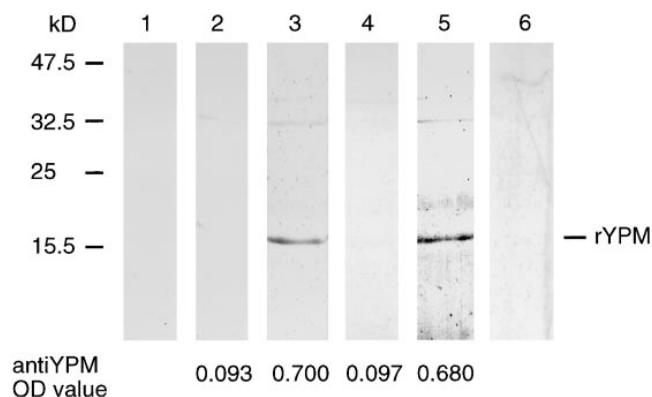
Figure 3. Western blot analysis of the two patients' sera. 1.0 \mu g of rYPM (lanes 2–5), or rMBP as control (lanes 1 and 6), was electrophoresed and transferred to PVDF membrane. Sera obtained from patient 1 on day 6 (lanes 1 and 2) or day 21 (lane 3), and from the patient 2 on day 7 (lane 4) or day 16 (lanes 5 and 6) were diluted to 1:100 and applied to the membrane. Bound IgG was detected with peroxidase-conjugated F(ab) 2 fraction of rabbit anti-human IgG and analyzed with an image analyzing system. Molecular weight markers are noted on the left and rYPM is indicated on the right.
