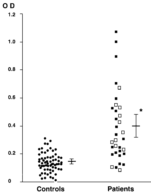
Figure 1. IgG anti-YPM antibodies in patients with Y. pseudotuberculosis infection measured by ELISA. The sera obtained from IVGG-treated ( \square ) or untreated ( \blacksquare ) patients and healthy children ( \bullet ) were diluted to 1:400 and applied to either an antigen-coated (5 \mu g/ml) or no antigen-coated well. In all experiments, OD of the no antigen-coated wells was < 0.01 and was subtracted from the OD of the antigen-coated wells. Each bar indicates the mean \pm 2 SEM. * P = 0.0001 by Student's t test.
