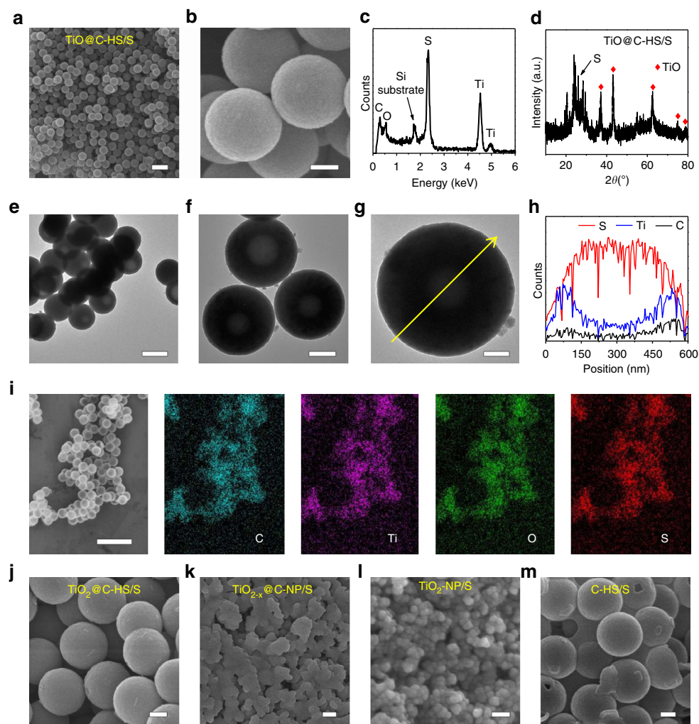
Figure 4 | Characterization of the sulfur-based composite materials. (a,b) SEM image, (c) EDX spectrum, (d) X-ray diffraction pattern, (e–g) TEM images, (h) linear distributions of S, Ti and C along the arrow line on g, and (i) EDX mapping area and corresponding elemental distributions of C, Ti, O and S of \text{TiO@C-HS/S} . SEM images of (j) \text{TiO}_2 @C-HS/S, (k) \text{TiO}_2-x @C-NP/S, (l) \text{TiO}_2 -NP/S and (m) C-HS/S. Scale bars, 1 \mu\text{m} (a), scale bars, 200 nm (b,f,j,k,m), scale bars, 500 nm (e), scale bars, 100 nm (g,l), scale bars, 2 \mu\text{m} (i).
