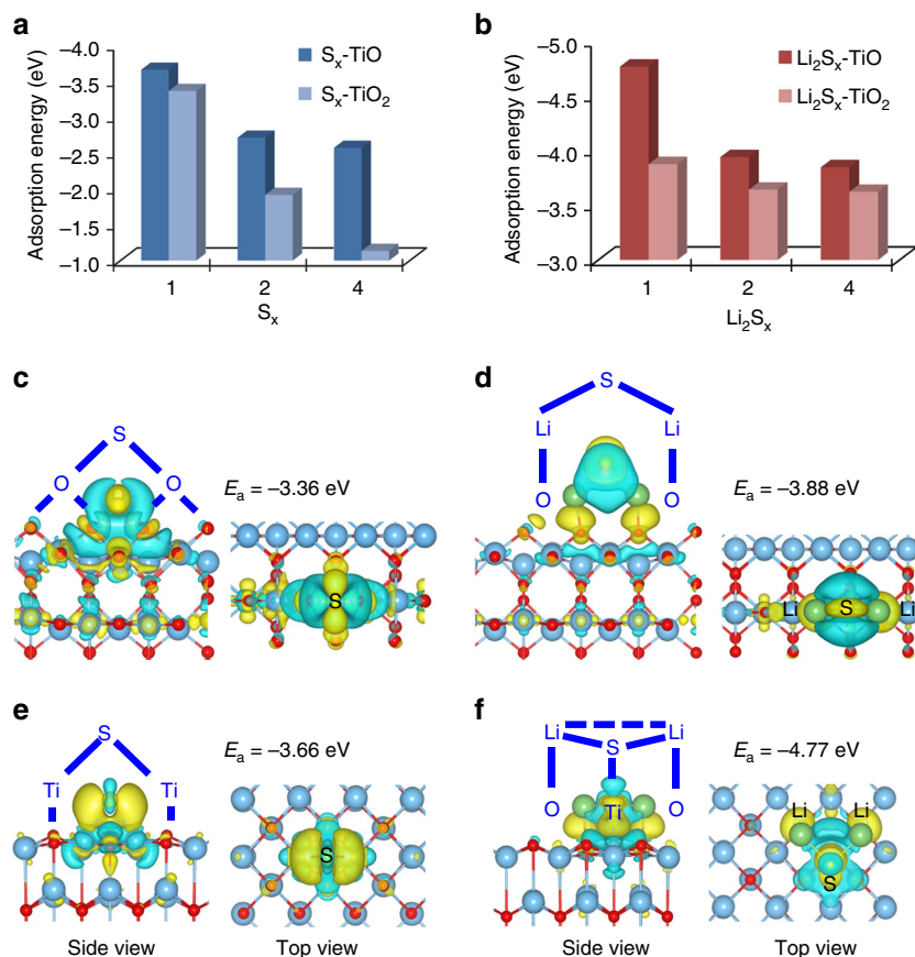
Figure 7 | DFT analysis of adsorption energies of S species on TiO (001) and TiO 2 (110). Adsorption energies for (a) S_x and (b) Li_2S_x ( x=1, 2 and 4) compounds on TiO (001) and TiO 2 (110) surfaces. Isosurface of the charge density difference for (c) S and (d) Li_2S adsorbed on TiO 2 (110), and (e) S and (f) Li_2S adsorbed on TiO (001). Yellow surfaces correspond to charge gains and blue surfaces correspond to an equivalent charge lost. To make the plot clear, the isovalues are defined as 0.002 in all cases.
