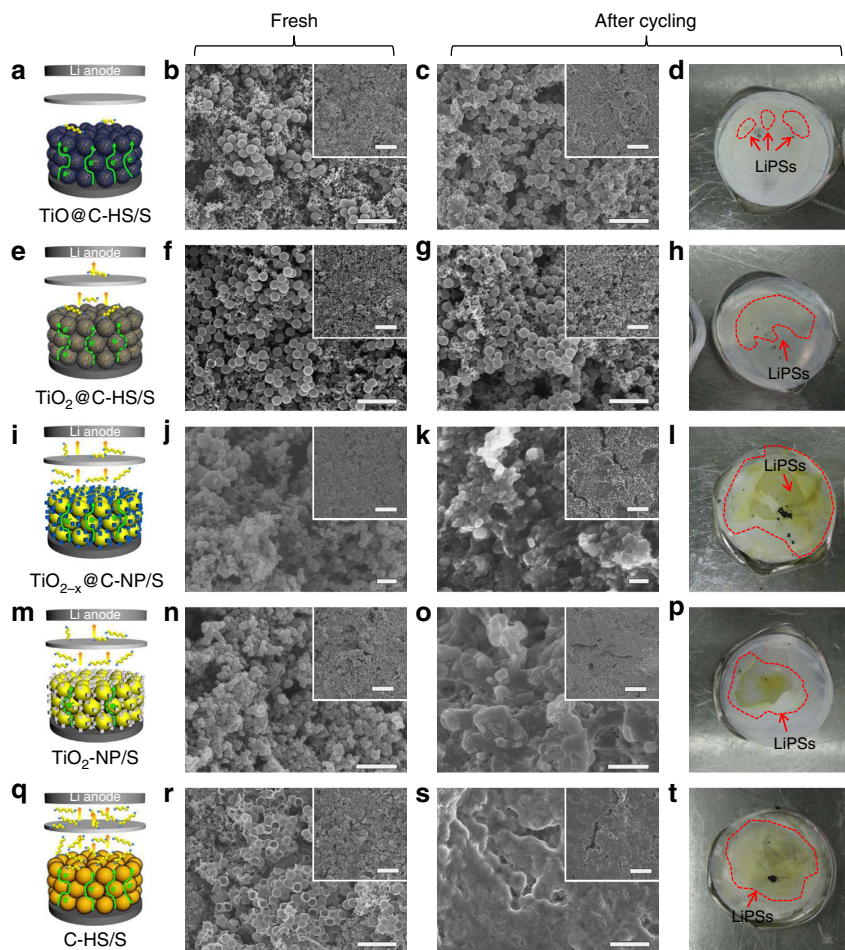
Figure 6 | Characterization of electrode films and separators during cycling. (a,e,i,m,q) Schematic illustration of the mechanisms during redox reaction, SEM images of (b,f,j,n,r) fresh electrode films, (c,g,k,o,s) cycled electrode films and (d,h,l,p,t) digital photos of cycled separators of (a-d) TiO@C-HS/S, (e-h) TiO 2 @C-HS/S, (i-l) TiO 2-x @C-NP/S, (m-p) TiO 2 -NP/S, and (q-t) C-HS/S. Scale bars, 2 μm (b,c,f,g,r,s), scale bars, 200 nm (j,k), scale bars, 500 nm (n,o), scale bars, 10 μm (insets of (b,c,f,g,j,k,n,o,r,s)).
