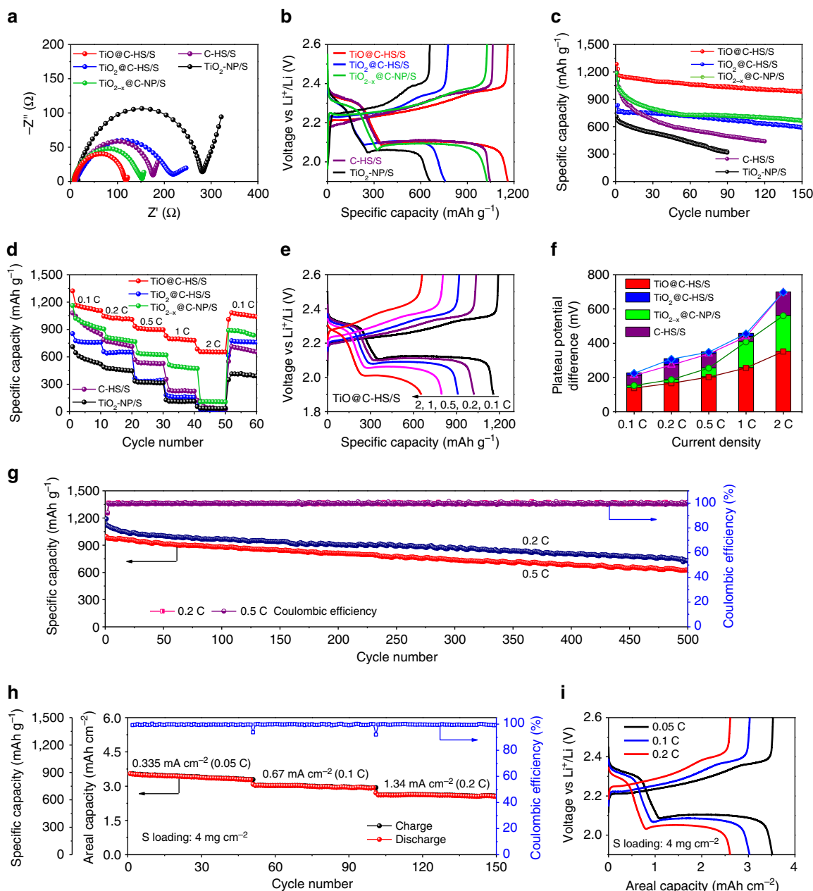
Figure 5 | Electrochemical evaluation of TiO@C-HS/S. (a) Nyquist plots before cycling from 1 MHz to 100 mHz, (b) the second-cycle galvanostatic charge/discharge voltage profiles at 0.1C, (c) cycle performances at 0.1C, (d) rate capabilities and (f) the potential differences between the charge and discharge plateaus at various current densities of the TiO@C-HS/S, TiO 2 @C-HS/S, TiO 2-x @C-NP/S, C-HS/S and TiO 2 -NP/S electrodes. (e) Voltage profiles at various current densities from 0.1 to 2 C and (g) prolonged cycle life and Coulombic efficiency at 0.2 and 0.5 C of the TiO@C-HS/S electrode. (h) Areal capacities and (i) voltage profiles at various current densities from 0.335 (0.05 C) to 1.34 mA cm -2 (0.2 C) of the TiO@C-HS/S electrode with high sulfur mass loading of 4.0 mg cm -2 .
