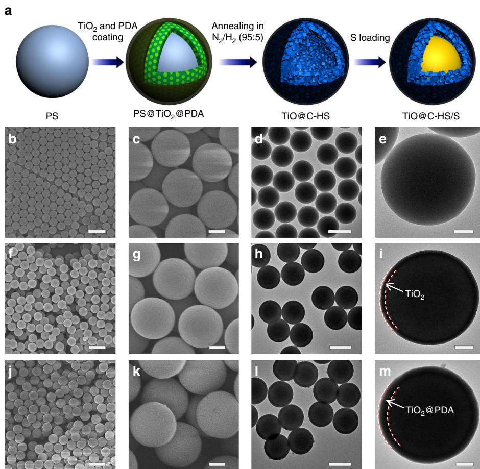
Figure 2 | Synthesis process of the TiO@C-HS/S composite. (a) Schematic illustration of the synthesis process of the TiO@C-HS/S composite. SEM and TEM images of (b–e) PS spheres, (f–i) PS@ TiO_2 core-shell spheres and (j–m) PS@ TiO_2 @PDA spheres. Scale bars, 1 \mu m (b,f,j), scale bars, 200 nm (c,g,k), scale bars, 500 nm (d,h,l), scale bars, 100 nm (e,i,m).
