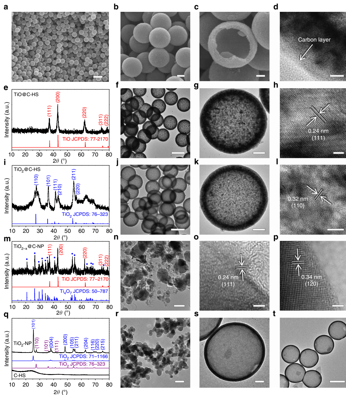
Figure 3 | Characterization of TiO@C-HS and other control host materials. (a–c) SEM images, (e,i,m,q) X-ray diffraction patterns, (d,f,h-j,l,n-p,r-t) TEM images of (a–h) TiO@C-HS, (i–l) TiO 2 @C-HS, (m–p) TiO 2-x @C-NP, (q,r) TiO 2 -NP and (s,t) C-HS. Scale bars, 1 \mu m (a), scale bars, 200 nm (b), scale bars, 100 nm (c,g,k,n,s), scale bars, 500 nm (f,j,t), scale bars, 10 nm (d), scale bars, 5 nm (l), scale bars, 2 nm (h,o,p), scale bars, 50 nm (r). a.u., arbitrary unit.
